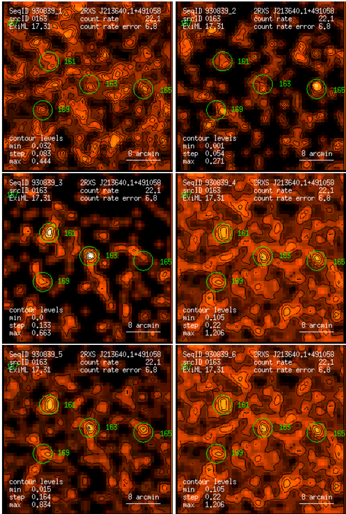
Figure 163: RASS 930839: detection 0163: band rate images, Gaussian filter: (1) PSPC channels 11 – 41, (2) 52 – 90, (3) 91 – 201, (4) 11 – 235, (5) 52 – 201, (6) 11 – 201. Broad band rates in counts/ks. Band rate contour levels in counts/ks/arcmin 2 .
