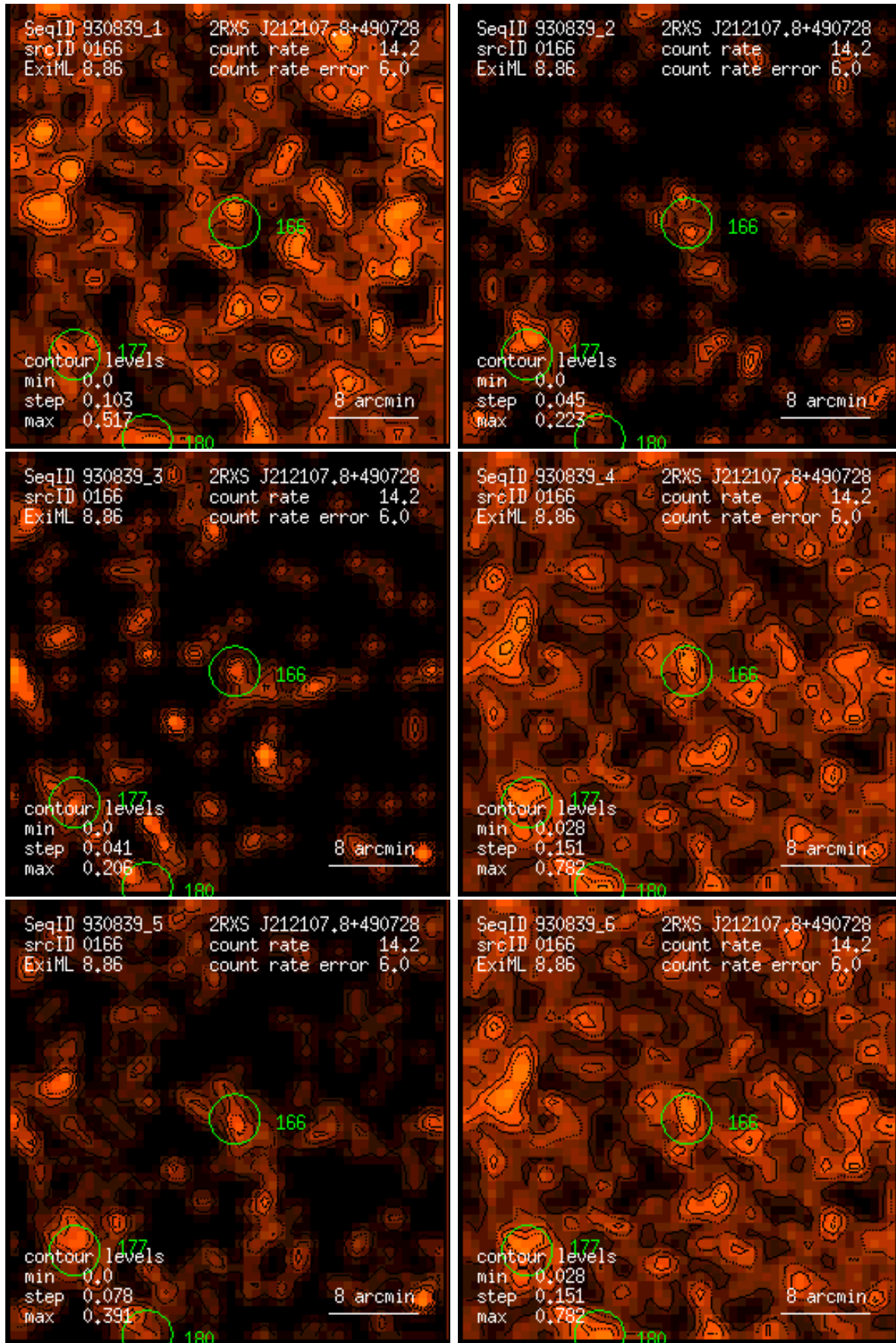
Figure 166: RASS 930839: detection 0166: band rate images, Gaussian filter: (1) PSPC channels 11 – 41, (2) 52 – 90, (3) 91 – 201, (4) 11 – 235, (5) 52 – 201, (6) 11 – 201. Broad band rates in counts/ks. Band rate contour levels in counts/ks/arcmin 2 .
