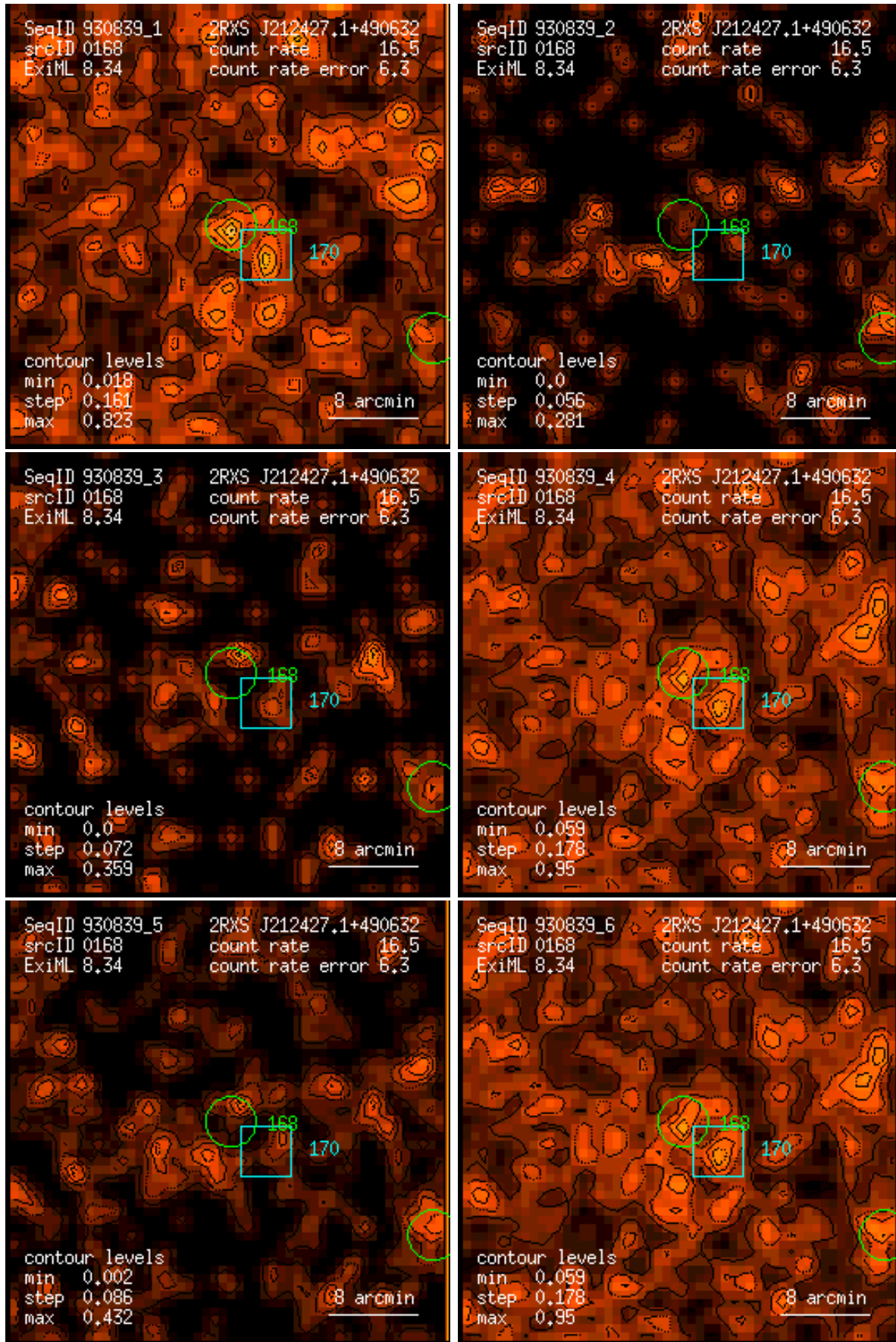
Figure 168: RASS 930839: detection 0168: band rate images, Gaussian filter: (1) PSPC channels 11 – 41, (2) 52 – 90, (3) 91 – 201, (4) 11 – 235, (5) 52 – 201, (6) 11 – 201. Broad band rates in counts/ks. Band rate contour levels in counts/ks/arcmin 2 .
