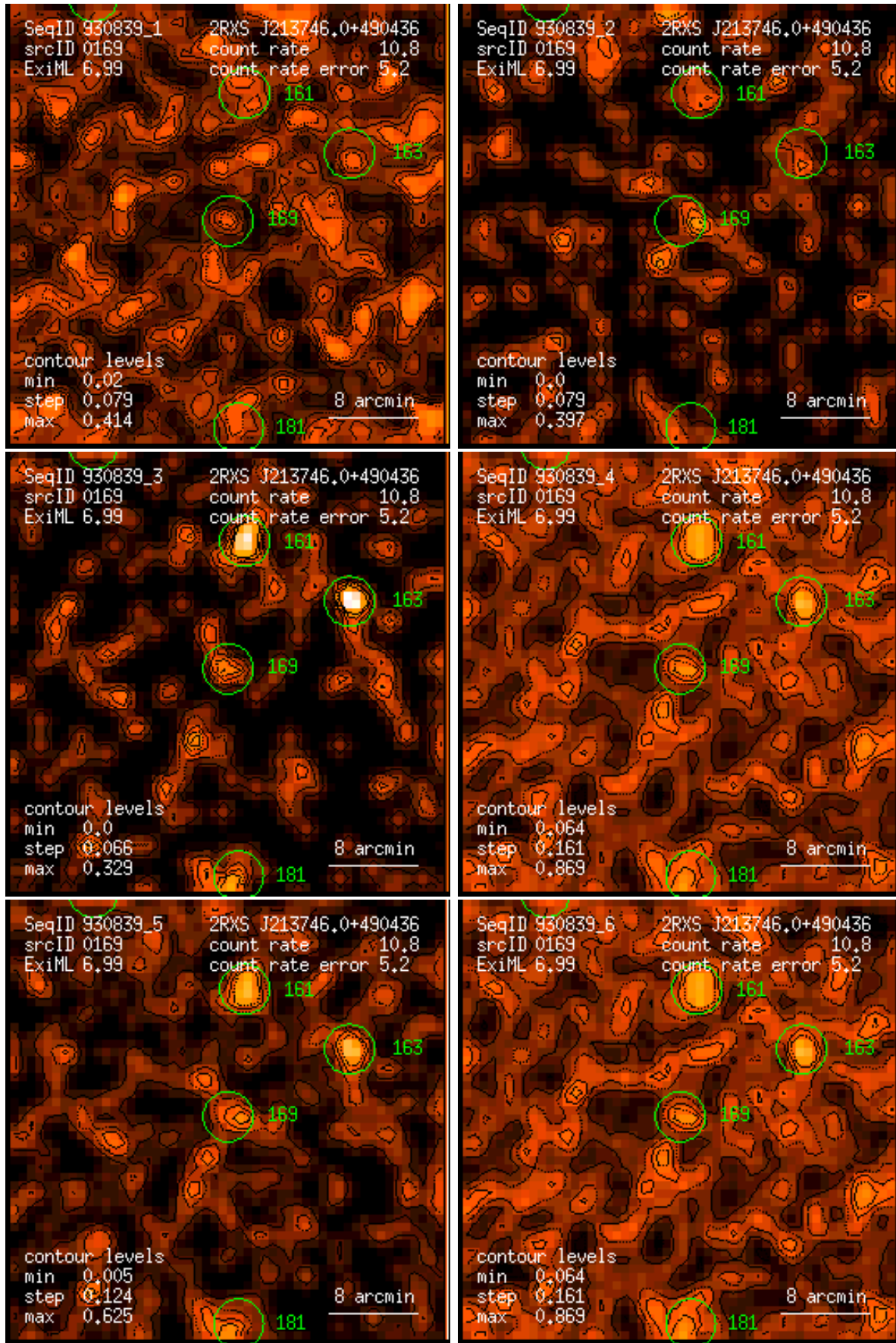
Figure 169: RASS 930839: detection 0169: band rate images, Gaussian filter: (1) PSPC channels 11 – 41, (2) 52 – 90, (3) 91 – 201, (4) 11 – 235, (5) 52 – 201, (6) 11 – 201. Broad band rates in counts/ks. Band rate contour levels in counts/ks/arcmin 2 .
