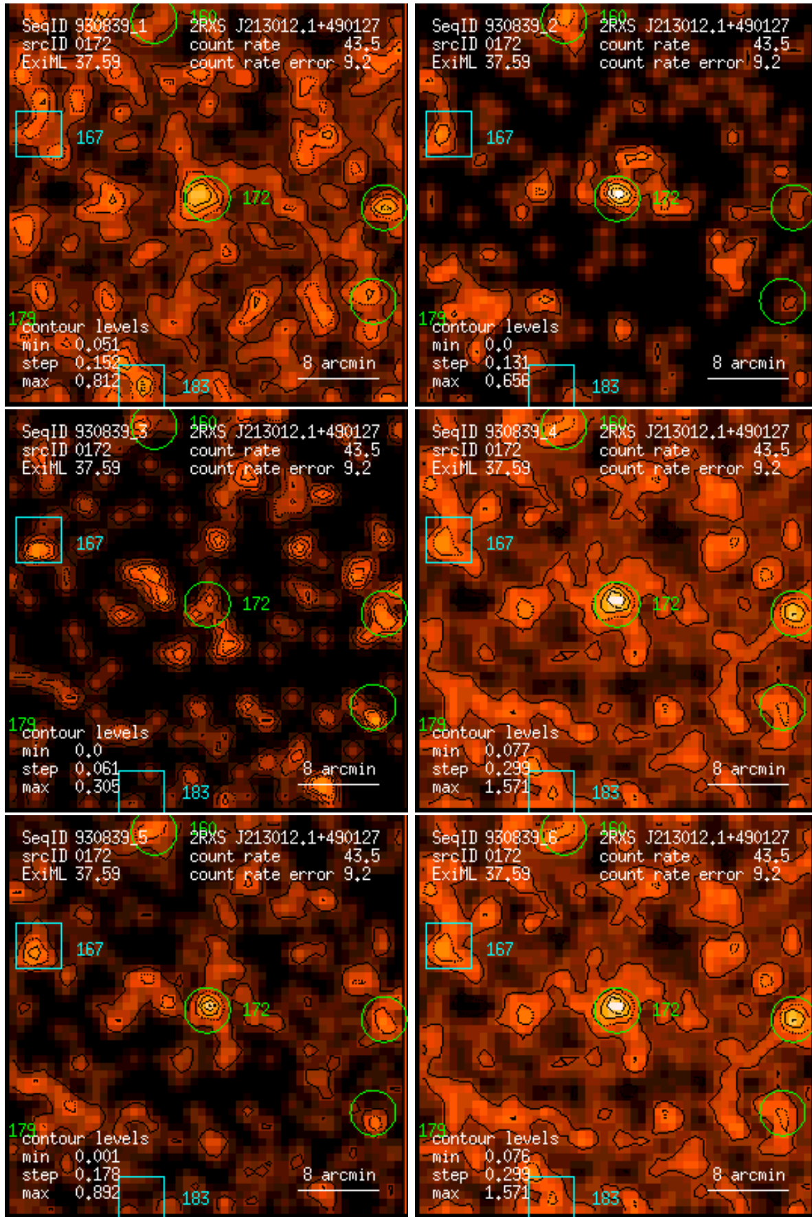
Figure 172: RASS 930839: detection 0172: band rate images, Gaussian filter: (1) PSPC channels 11 – 41, (2) 52 – 90, (3) 91 – 201, (4) 11 – 235, (5) 52 – 201, (6) 11 – 201. Broad band rates in counts/ks. Band rate contour levels in counts/ks/arcmin 2 .
