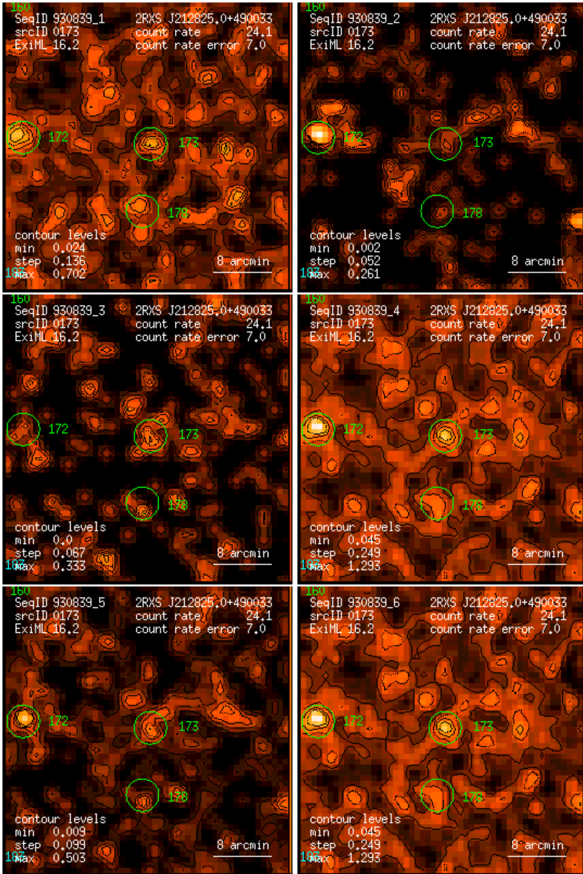
Figure 173: RASS 930839: detection 0173: band rate images, Gaussian filter: (1) PSPC channels 11 – 41, (2) 52 – 90, (3) 91 – 201, (4) 11 – 235, (5) 52 – 201, (6) 11 – 201. Broad band rates in counts/ks. Band rate contour levels in counts/ks/arcmin 2 .
