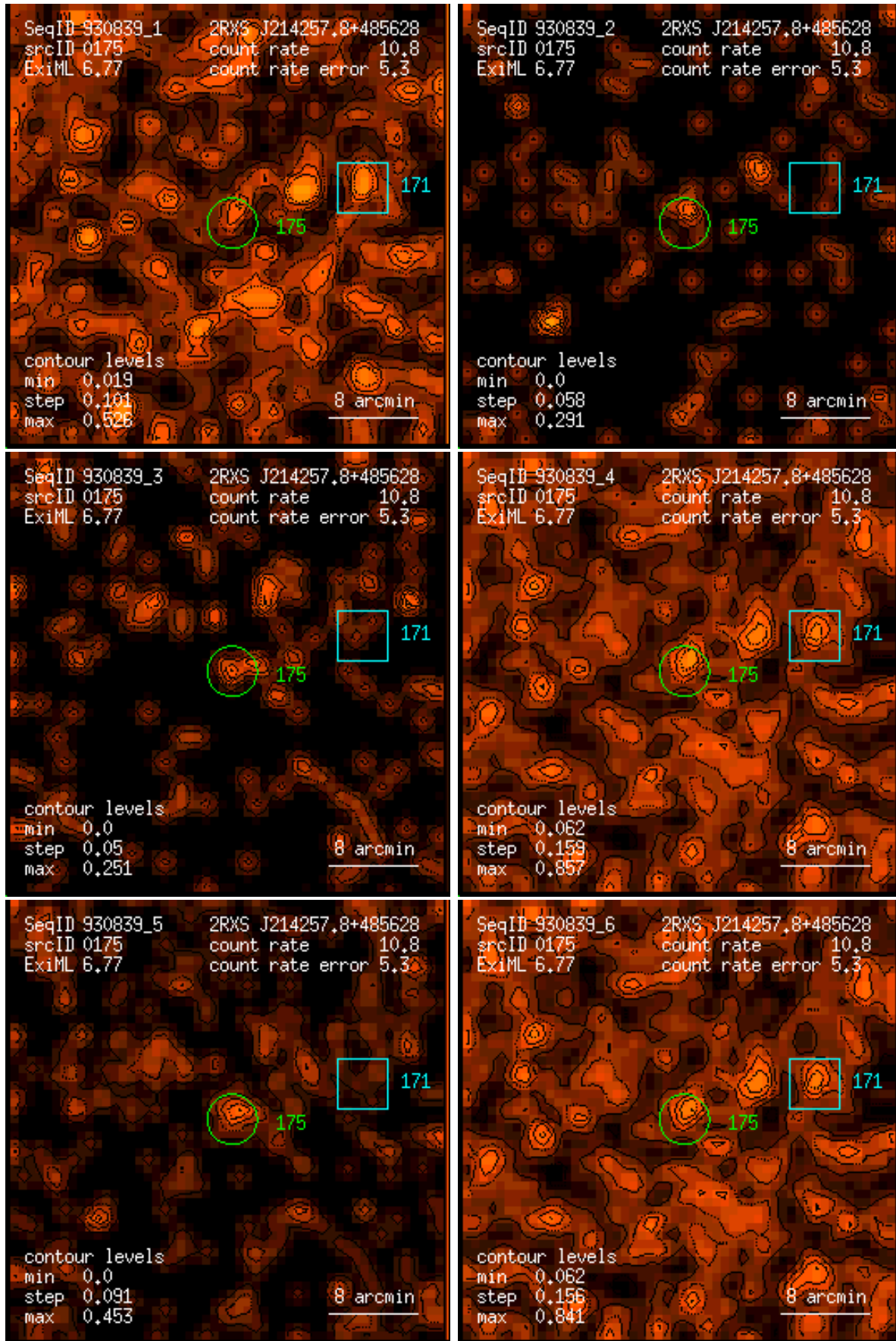
Figure 175: RASS 930839: detection 0175: band rate images, Gaussian filter: (1) PSPC channels 11 – 41, (2) 52 – 90, (3) 91 – 201, (4) 11 – 235, (5) 52 – 201, (6) 11 – 201. Broad band rates in counts/ks. Band rate contour levels in counts/ks/arcmin 2 .
