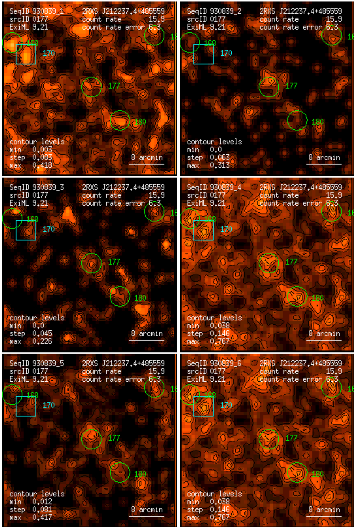
Figure 177: RASS 930839: detection 0177: band rate images, Gaussian filter: (1) PSPC channels 11 – 41, (2) 52 – 90, (3) 91 – 201, (4) 11 – 235, (5) 52 – 201, (6) 11 – 201. Broad band rates in counts/ks. Band rate contour levels in counts/ks/arcmin 2 .
