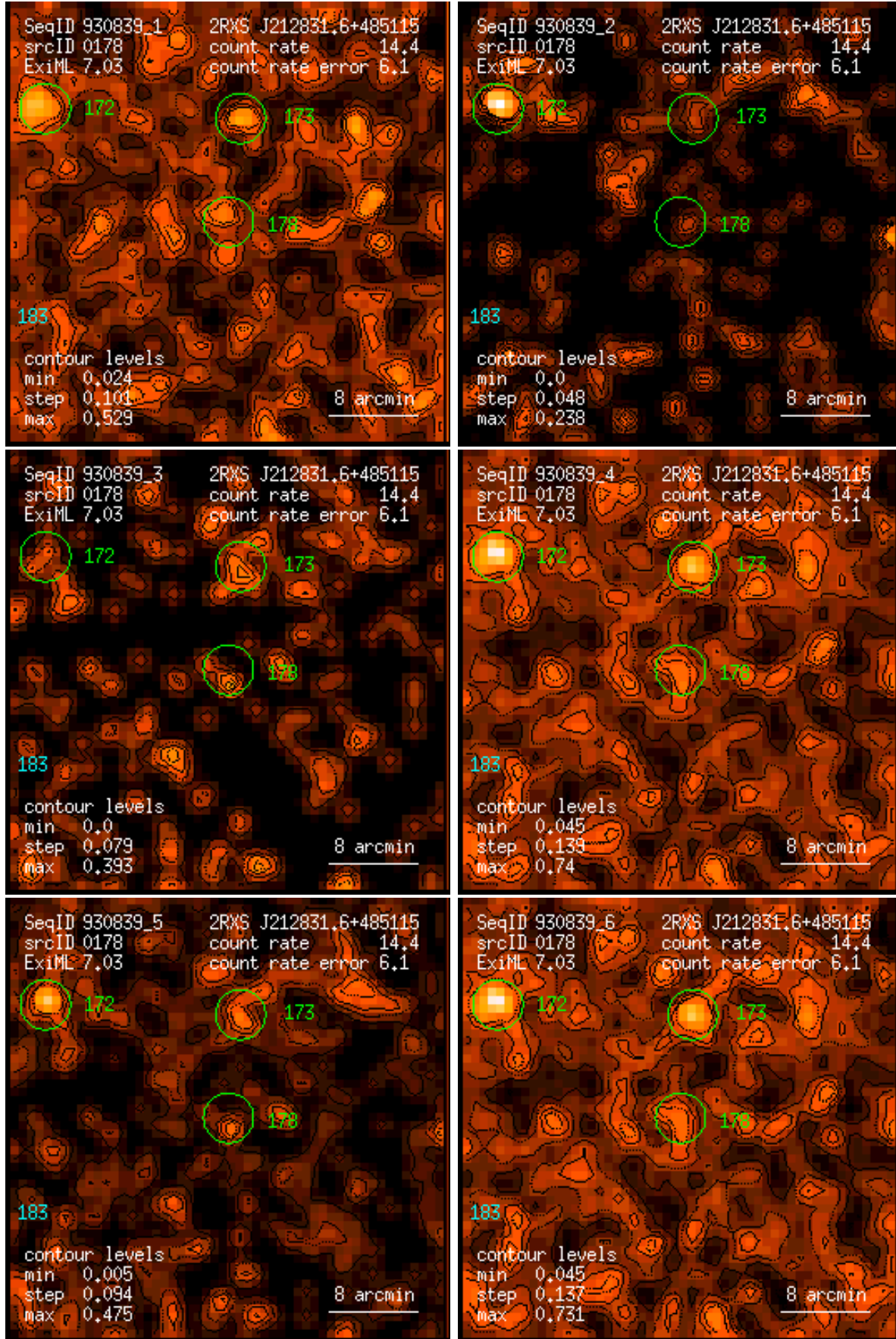
Figure 178: RASS 930839: detection 0178: band rate images, Gaussian filter: (1) PSPC channels 11 – 41, (2) 52 – 90, (3) 91 – 201, (4) 11 – 235, (5) 52 – 201, (6) 11 – 201. Broad band rates in counts/ks. Band rate contour levels in counts/ks/arcmin 2 .
