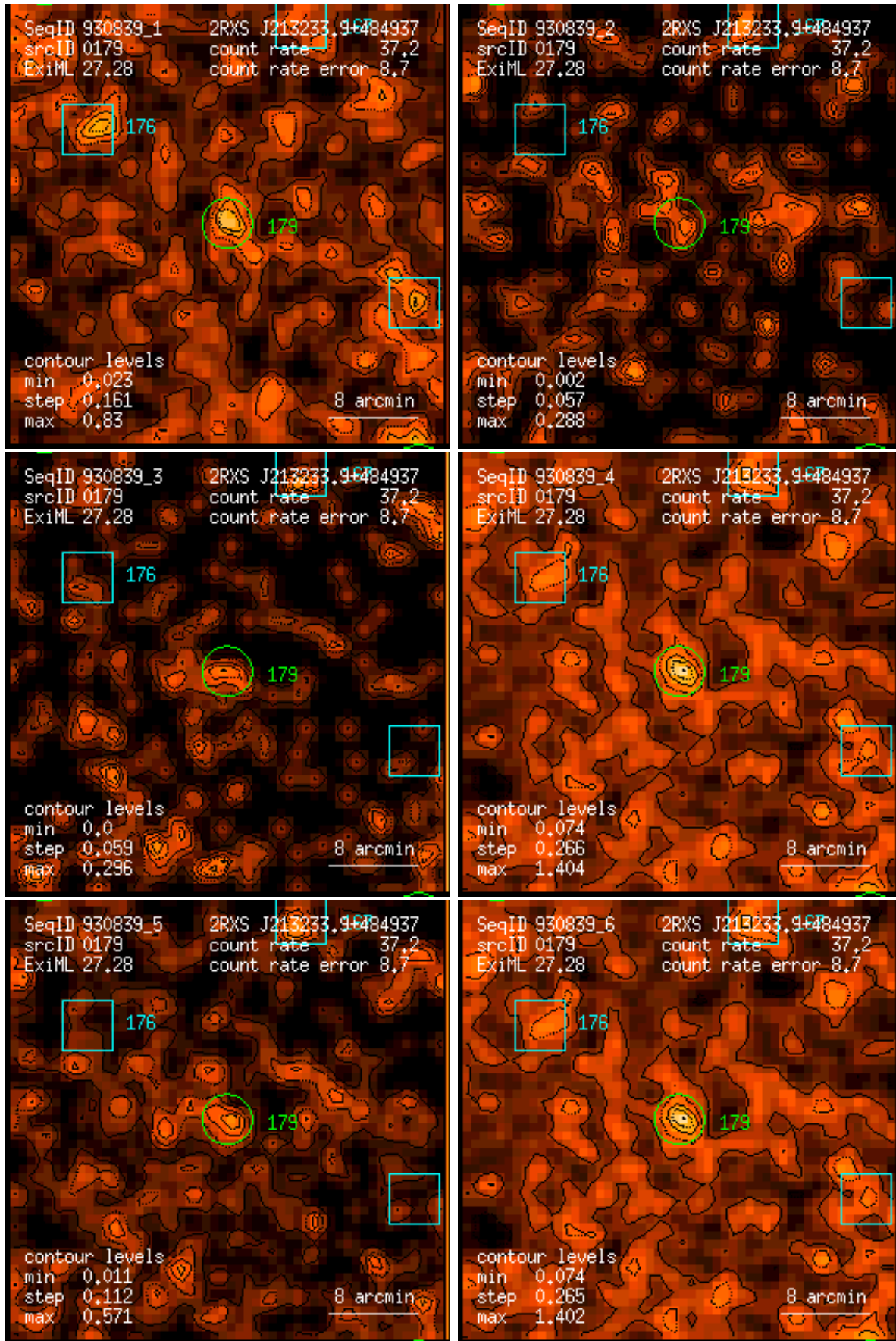
Figure 179: RASS 930839: detection 0179: band rate images, Gaussian filter: (1) PSPC channels 11 – 41, (2) 52 – 90, (3) 91 – 201, (4) 11 – 235, (5) 52 – 201, (6) 11 – 201. Broad band rates in counts/ks. Band rate contour levels in counts/ks/arcmin 2 .
