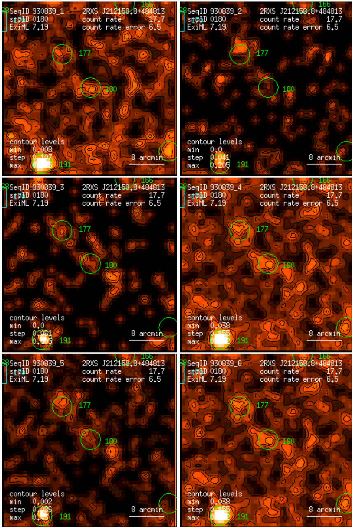
Figure 180: RASS 930839: detection 0180: band rate images, Gaussian filter: (1) PSPC channels 11 – 41, (2) 52 – 90, (3) 91 – 201, (4) 11 – 235, (5) 52 – 201, (6) 11 – 201. Broad band rates in counts/ks. Band rate contour levels in counts/ks/arcmin 2 .
