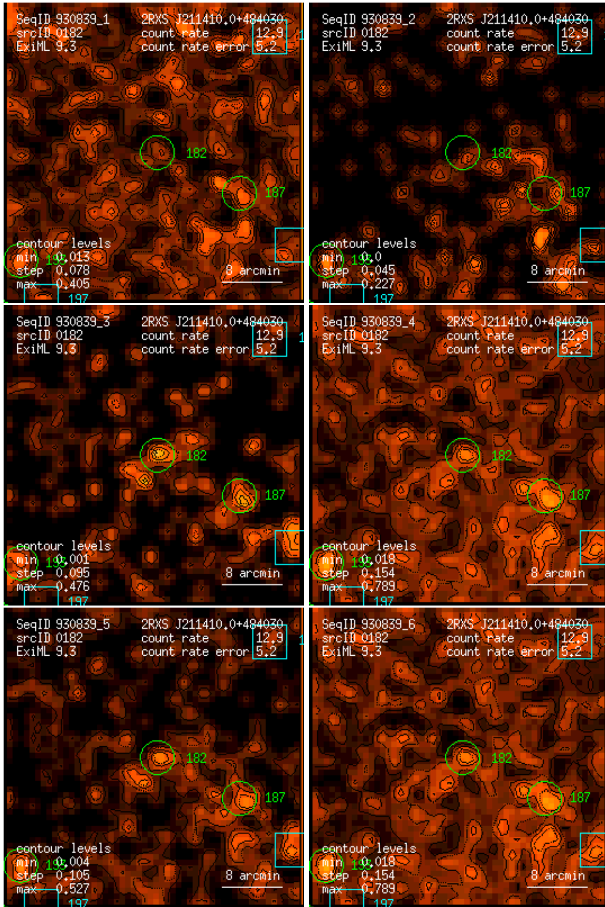
Figure 182: RASS 930839: detection 0182: band rate images, Gaussian filter: (1) PSPC channels 11 – 41, (2) 52 – 90, (3) 91 – 201, (4) 11 – 235, (5) 52 – 201, (6) 11 – 201. Broad band rates in counts/ks. Band rate contour levels in counts/ks/arcmin 2 .
