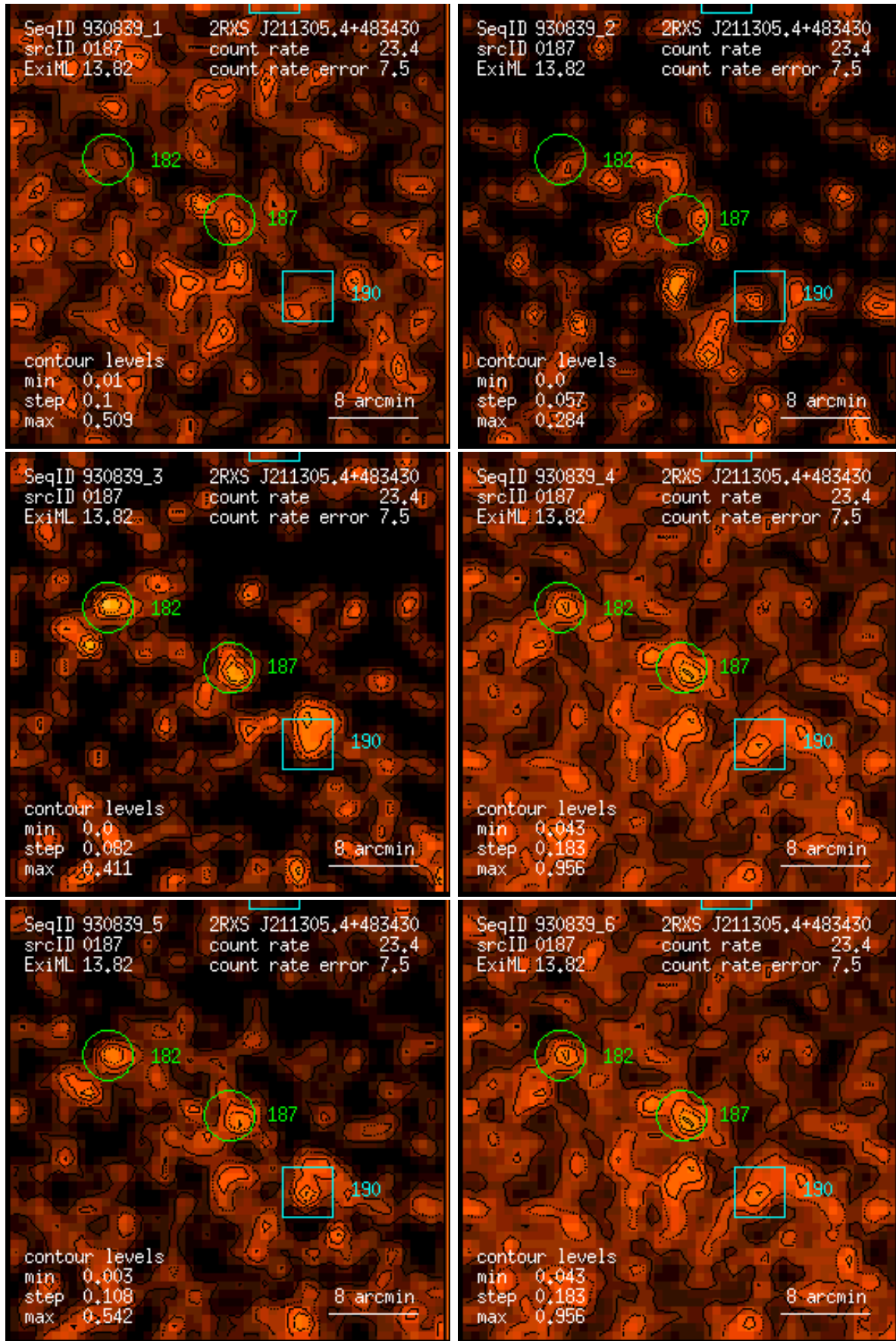
Figure 187: RASS 930839: detection 0187: band rate images, Gaussian filter: (1) PSPC channels 11 – 41, (2) 52 – 90, (3) 91 – 201, (4) 11 – 235, (5) 52 – 201, (6) 11 – 201. Broad band rates in counts/ks. Band rate contour levels in counts/ks/arcmin 2 .
