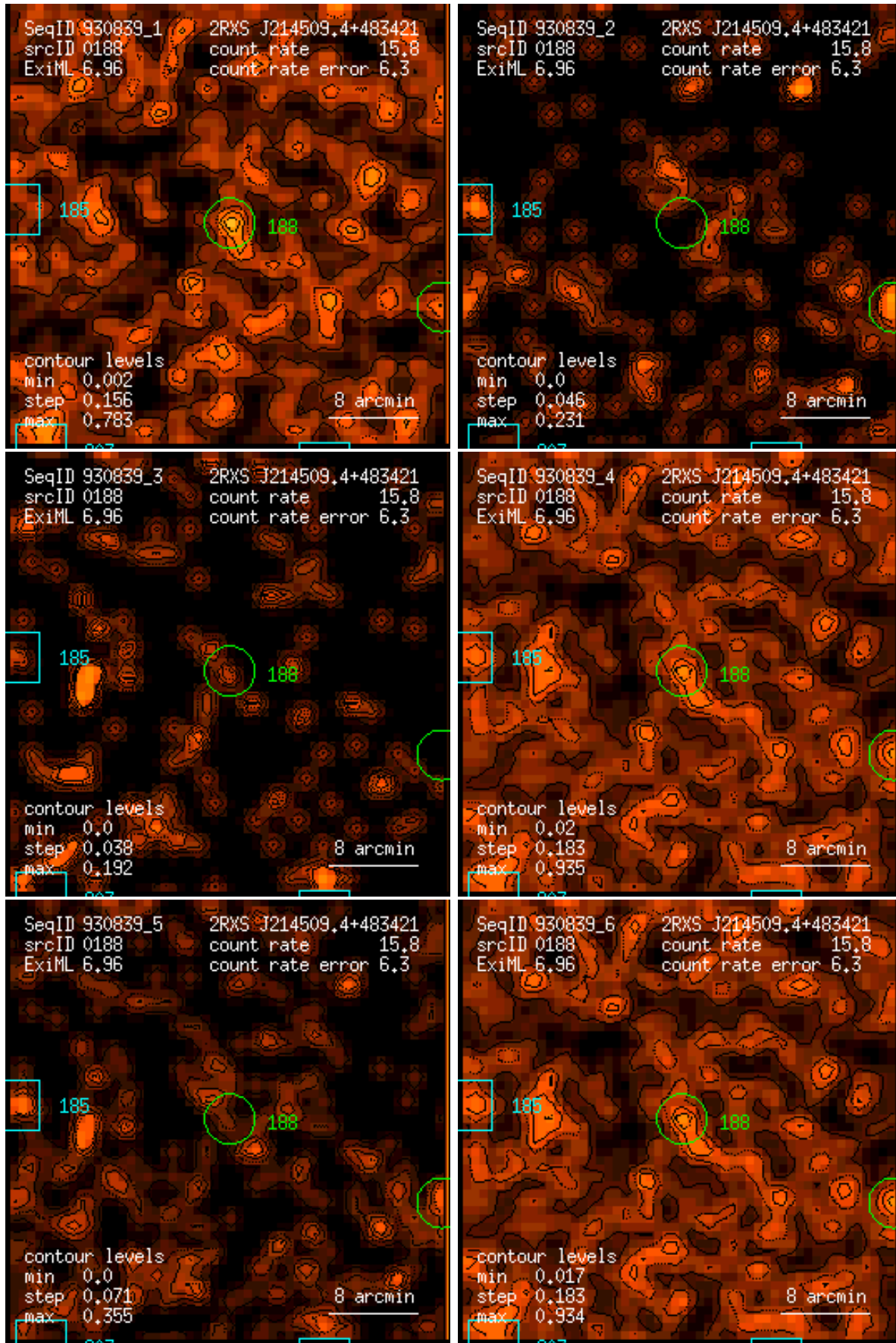
Figure 188: RASS 930839: detection 0188: band rate images, Gaussian filter: (1) PSPC channels 11 – 41, (2) 52 – 90, (3) 91 – 201, (4) 11 – 235, (5) 52 – 201, (6) 11 – 201. Broad band rates in counts/ks. Band rate contour levels in counts/ks/arcmin 2 .
