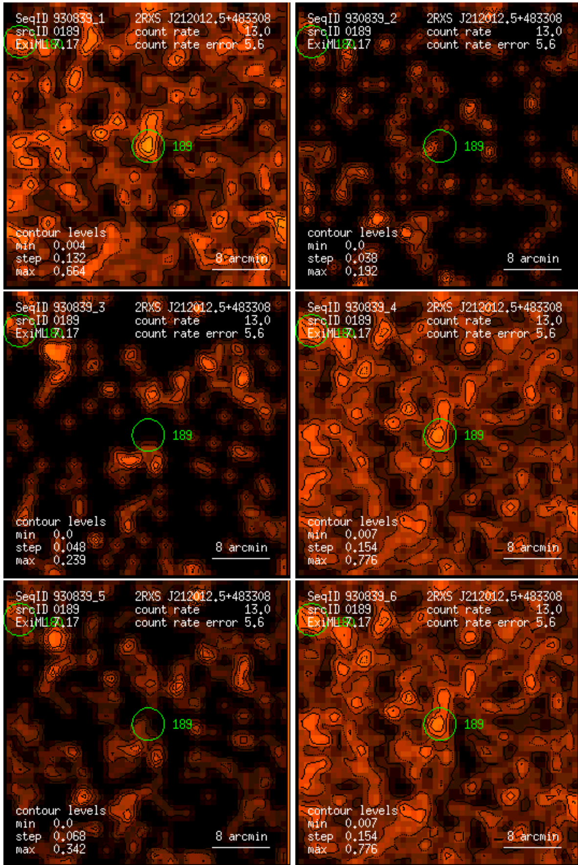
Figure 189: RASS 930839: detection 0189: band rate images, Gaussian filter: (1) PSPC channels 11 – 41, (2) 52 – 90, (3) 91 – 201, (4) 11 – 235, (5) 52 – 201, (6) 11 – 201. Broad band rates in counts/ks. Band rate contour levels in counts/ks/arcmin 2 .
