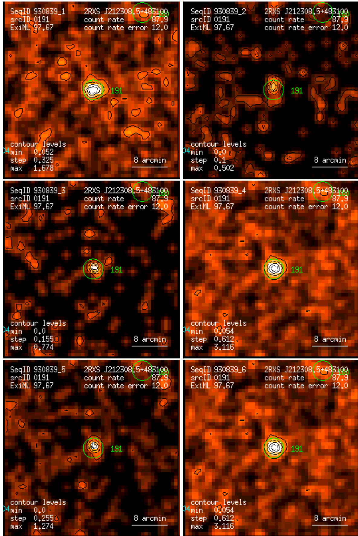
Figure 191: RASS 930839: detection 0191: band rate images, Gaussian filter: (1) PSPC channels 11 – 41, (2) 52 – 90, (3) 91 – 201, (4) 11 – 235, (5) 52 – 201, (6) 11 – 201. Broad band rates in counts/ks. Band rate contour levels in counts/ks/arcmin 2 .
