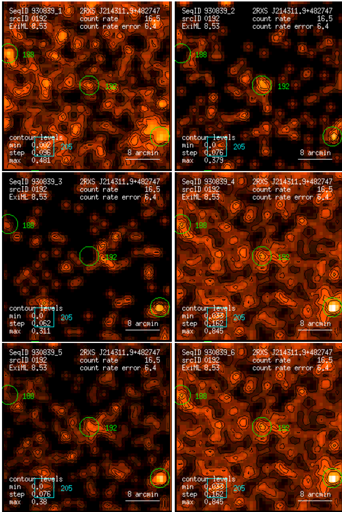
Figure 192: RASS 930839: detection 0192: band rate images, Gaussian filter: (1) PSPC channels 11 – 41, (2) 52 – 90, (3) 91 – 201, (4) 11 – 235, (5) 52 – 201, (6) 11 – 201. Broad band rates in counts/ks. Band rate contour levels in counts/ks/arcmin 2 .
