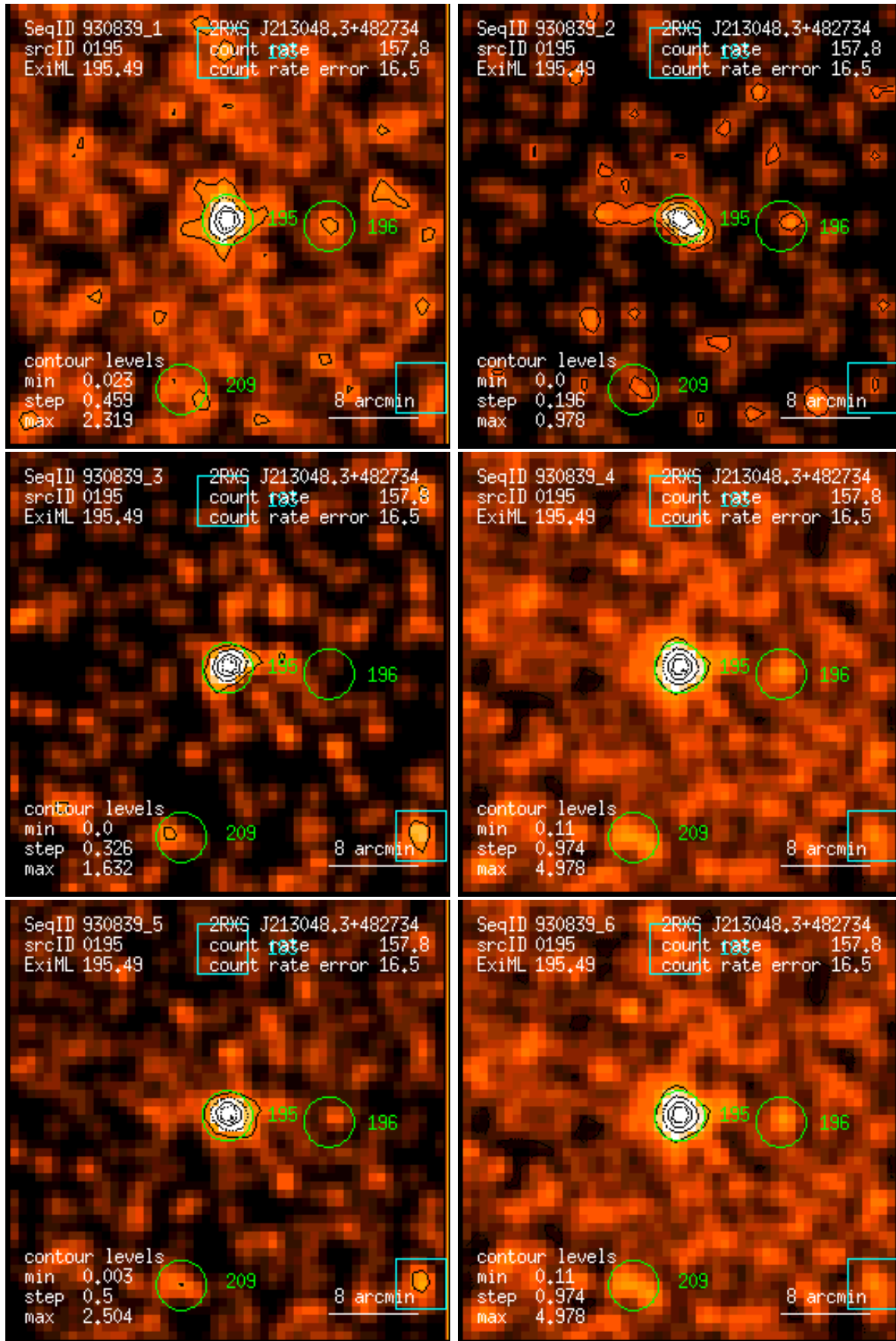
Figure 195: RASS 930839: detection 0195: band rate images, Gaussian filter: (1) PSPC channels 11 – 41, (2) 52 – 90, (3) 91 – 201, (4) 11 – 235, (5) 52 – 201, (6) 11 – 201. Broad band rates in counts/ks. Band rate contour levels in counts/ks/arcmin 2 .
