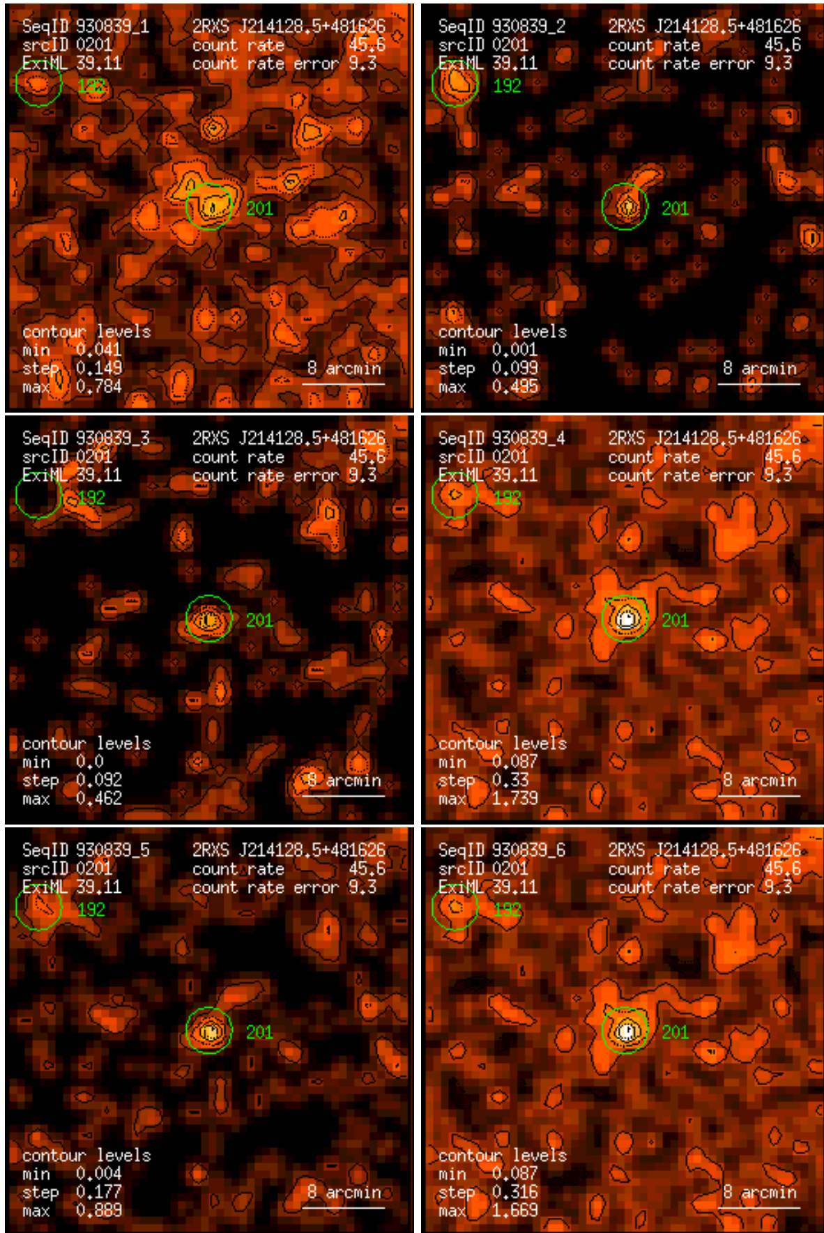
Figure 201: RASS 930839: detection 0201: band rate images, Gaussian filter: (1) PSPC channels 11 – 41, (2) 52 – 90, (3) 91 – 201, (4) 11 – 235, (5) 52 – 201, (6) 11 – 201. Broad band rates in counts/ks. Band rate contour levels in counts/ks/arcmin 2 .
