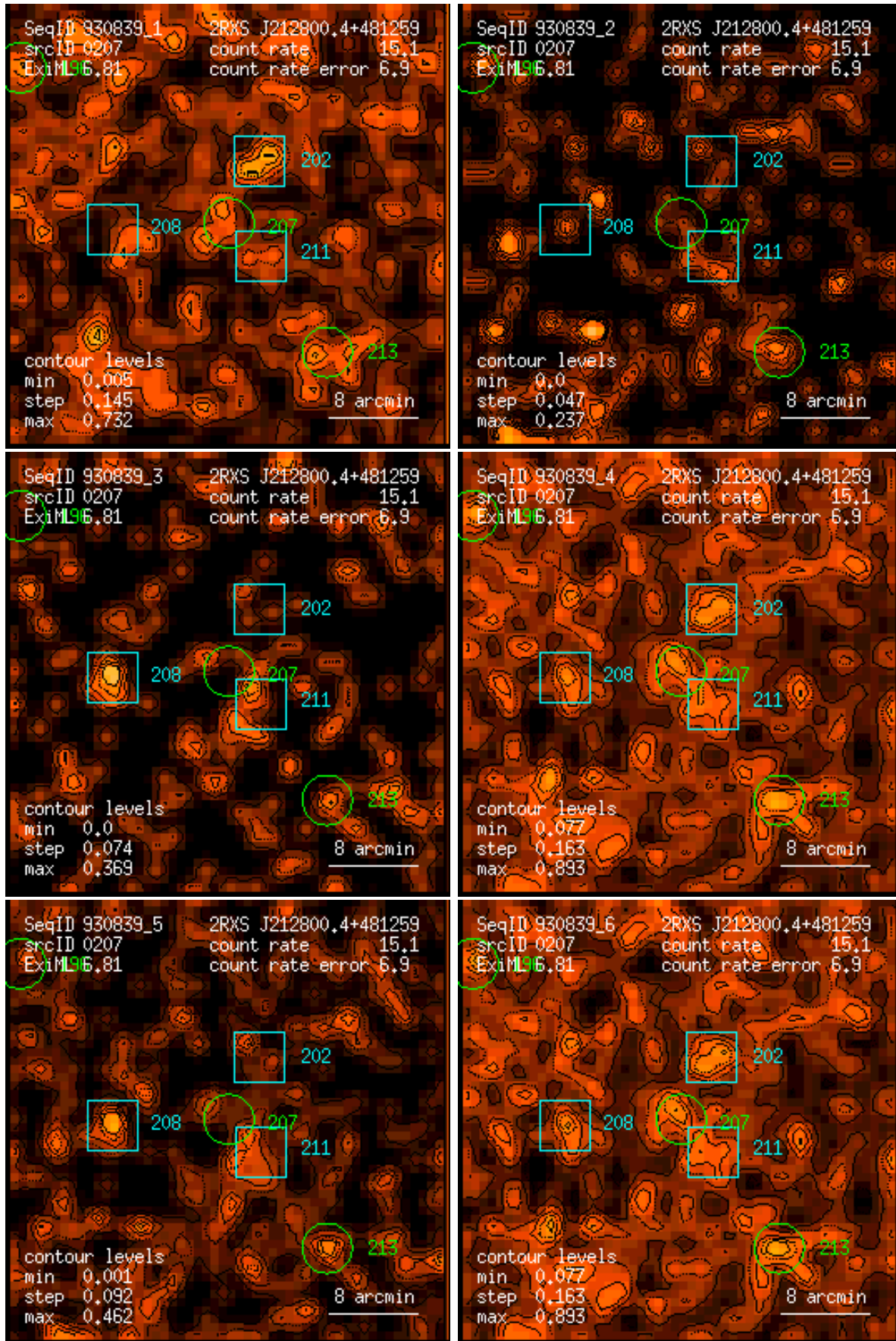
Figure 207: RASS 930839: detection 0207: band rate images, Gaussian filter: (1) PSPC channels 11 – 41, (2) 52 – 90, (3) 91 – 201, (4) 11 – 235, (5) 52 – 201, (6) 11 – 201. Broad band rates in counts/ks. Band rate contour levels in counts/ks/arcmin 2 .
