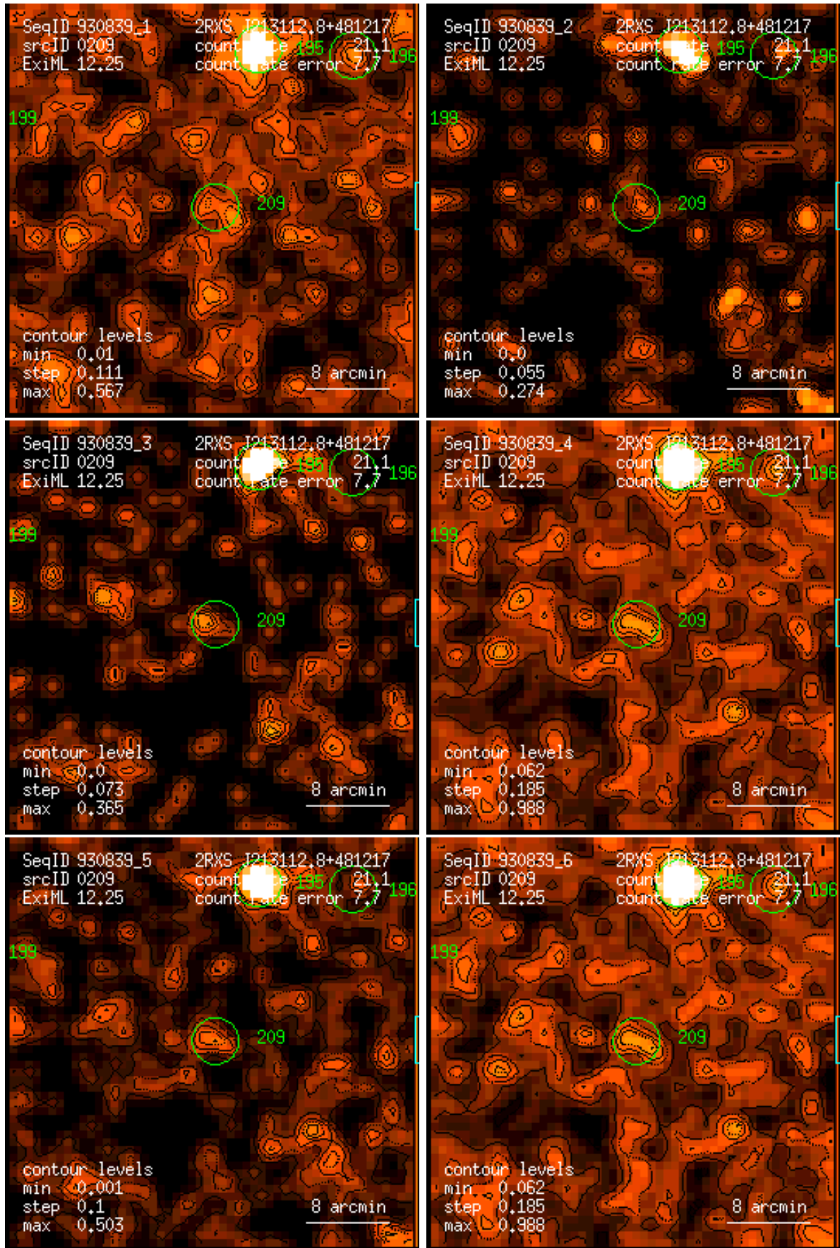
Figure 209: RASS 930839: detection 0209: band rate images, Gaussian filter: (1) PSPC channels 11 – 41, (2) 52 – 90, (3) 91 – 201, (4) 11 – 235, (5) 52 – 201, (6) 11 – 201. Broad band rates in counts/ks. Band rate contour levels in counts/ks/arcmin 2 .
