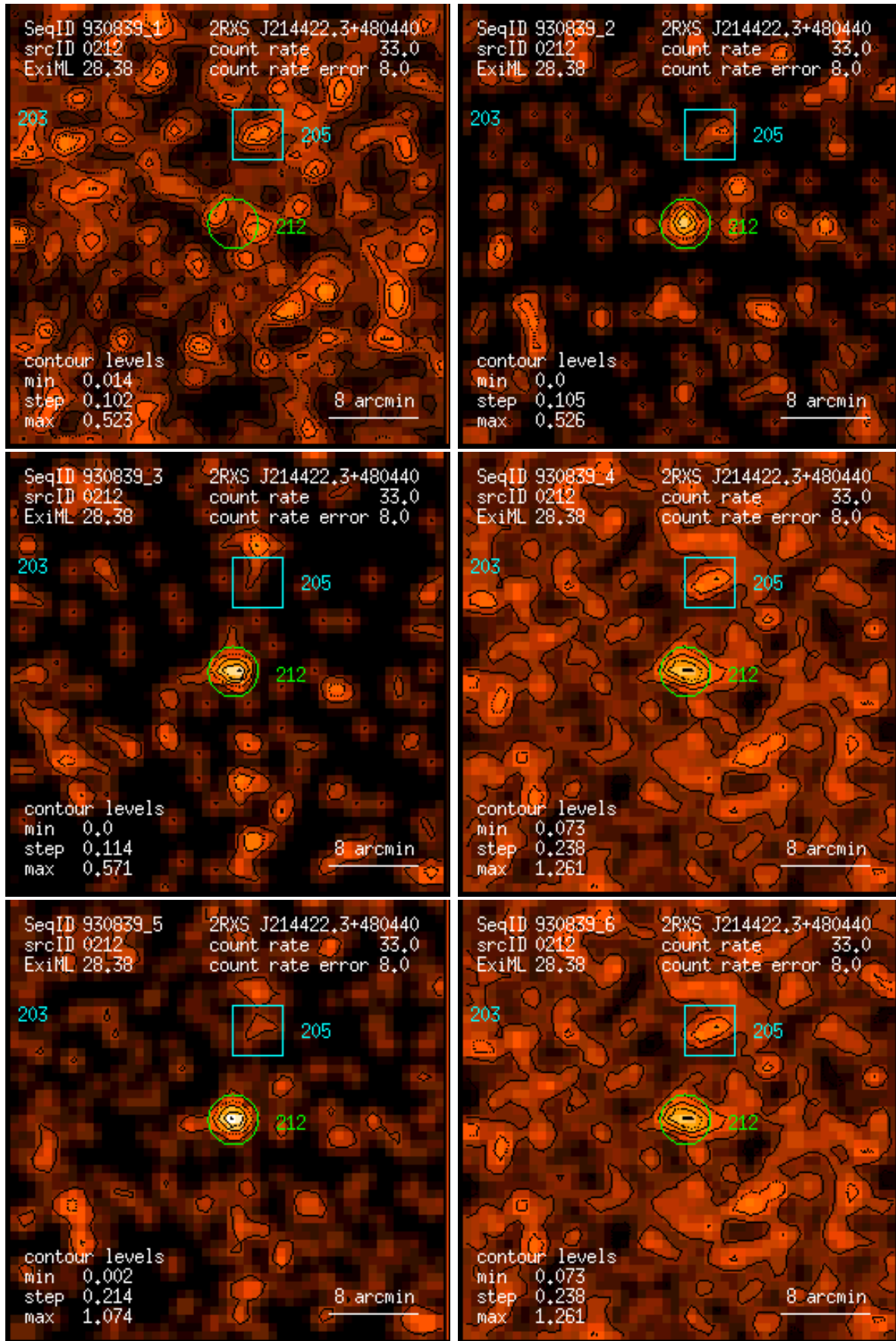
Figure 212: RASS 930839: detection 0212: band rate images, Gaussian filter: (1) PSPC channels 11 – 41, (2) 52 – 90, (3) 91 – 201, (4) 11 – 235, (5) 52 – 201, (6) 11 – 201. Broad band rates in counts/ks. Band rate contour levels in counts/ks/arcmin 2 .
