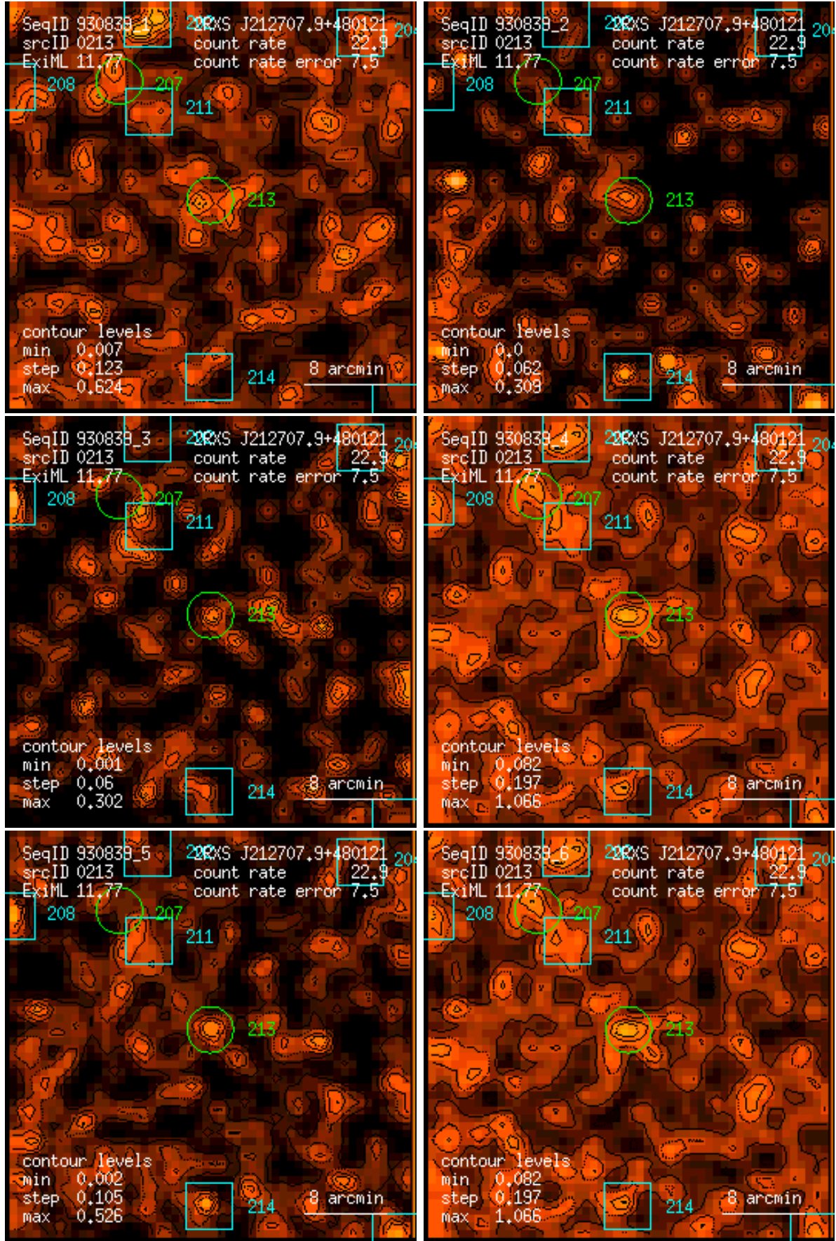
Figure 213: RASS 930839: detection 0213: band rate images, Gaussian filter: (1) PSPC channels 11 – 41, (2) 52 – 90, (3) 91 – 201, (4) 11 – 235, (5) 52 – 201, (6) 11 – 201. Broad band rates in counts/ks. Band rate contour levels in counts/ks/arcmin 2 .
