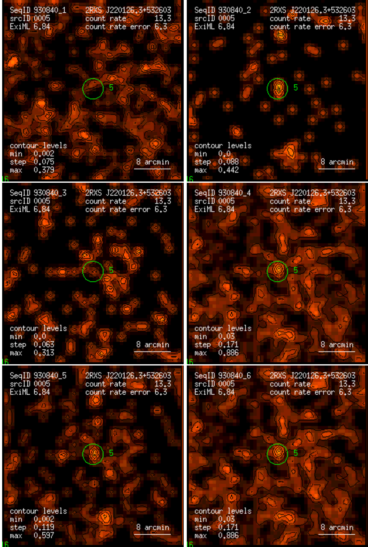
Figure 5: RASS 930840: detection 0005: band rate images, Gaussian filter: (1) PSPC channels 11 – 41, (2) 52 – 90, (3) 91 – 201, (4) 11 – 235, (5) 52 – 201, (6) 11 – 201. Broad band rates in counts/ks. Band rate contour levels in counts/ks/arcmin 2 .
