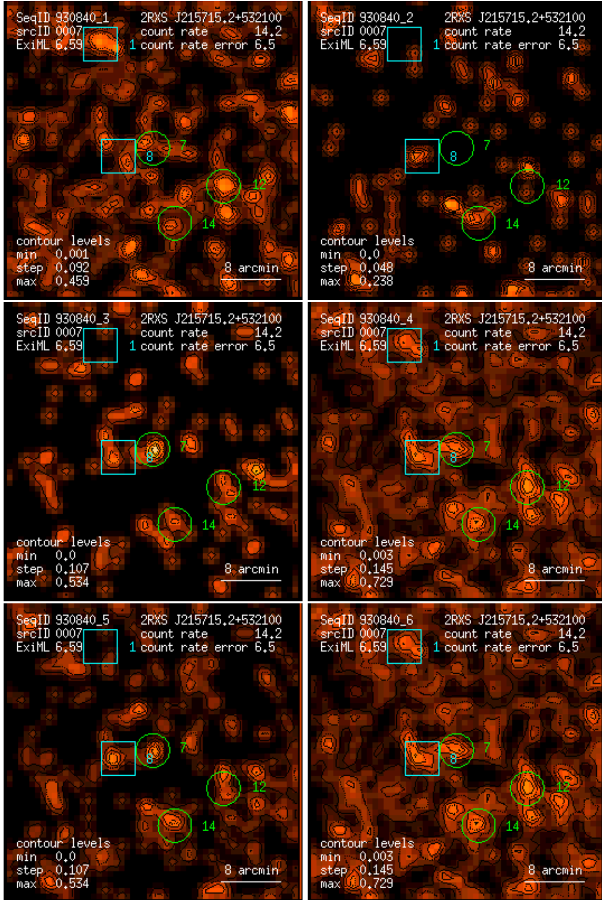
Figure 7: RASS 930840: detection 0007: band rate images, Gaussian filter: (1) PSPC channels 11 – 41, (2) 52 – 90, (3) 91 – 201, (4) 11 – 235, (5) 52 – 201, (6) 11 – 201. Broad band rates in counts/ks. Band rate contour levels in counts/ks/arcmin 2 .
