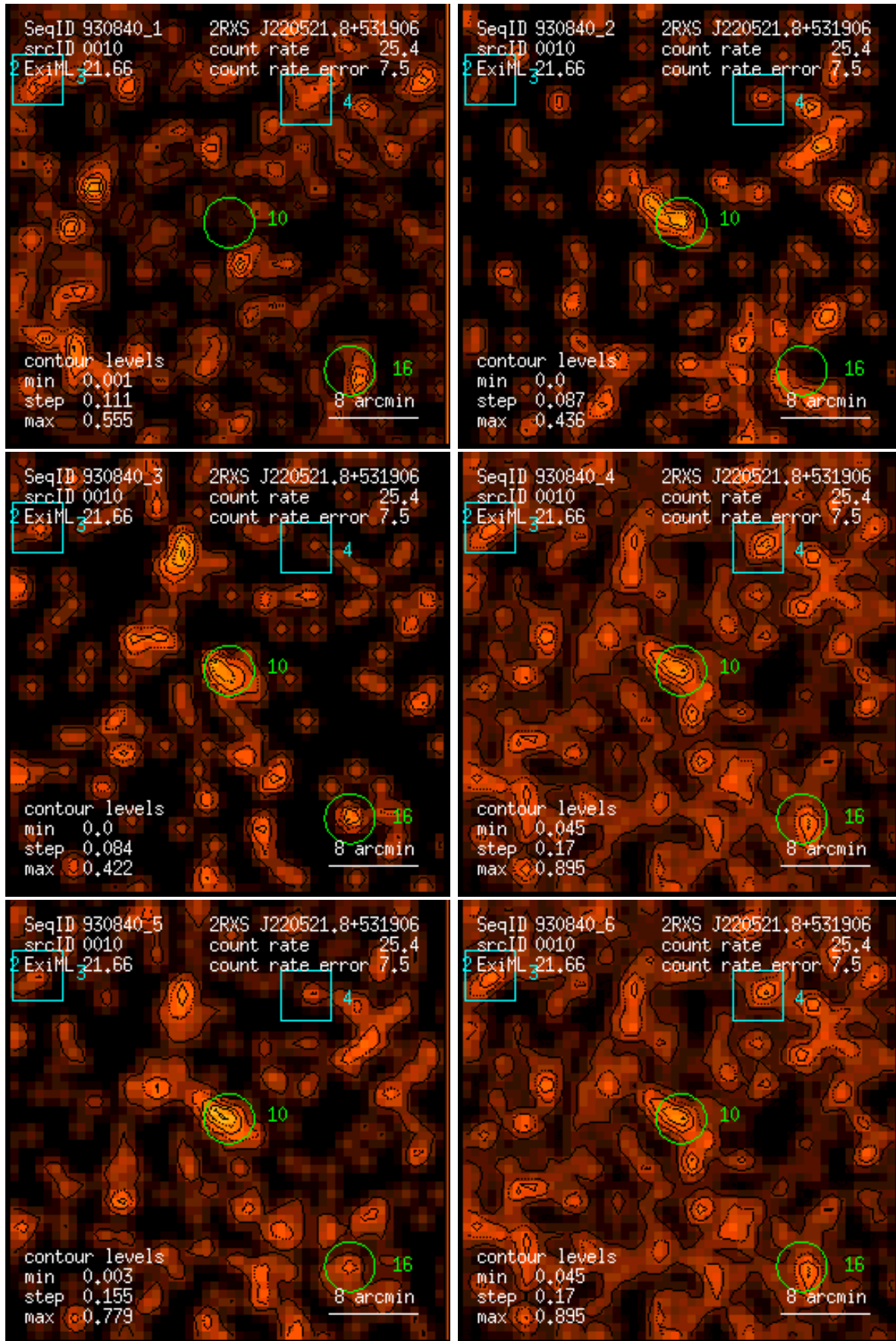
Figure 10: RASS 930840: detection 0010: band rate images, Gaussian filter: (1) PSPC channels 11 – 41, (2) 52 – 90, (3) 91 – 201, (4) 11 – 235, (5) 52 – 201, (6) 11 – 201. Broad band rates in counts/ks. Band rate contour levels in counts/ks/arcmin 2 .
