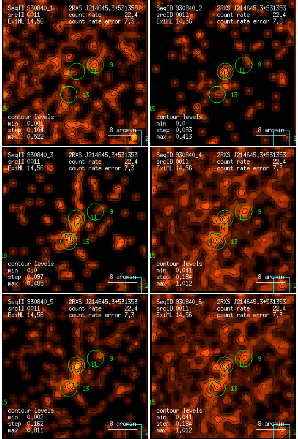
Figure 11: RASS 930840: detection 0011: band rate images, Gaussian filter: (1) PSPC channels 11 – 41, (2) 52 – 90, (3) 91 – 201, (4) 11 – 235, (5) 52 – 201, (6) 11 – 201. Broad band rates in counts/ks. Band rate contour levels in counts/ks/arcmin 2 .
