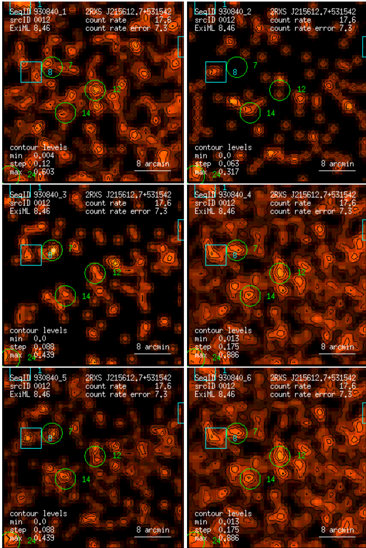
Figure 12: RASS 930840: detection 0012: band rate images, Gaussian filter: (1) PSPC channels 11 – 41, (2) 52 – 90, (3) 91 – 201, (4) 11 – 235, (5) 52 – 201, (6) 11 – 201. Broad band rates in counts/ks. Band rate contour levels in counts/ks/arcmin 2 .
