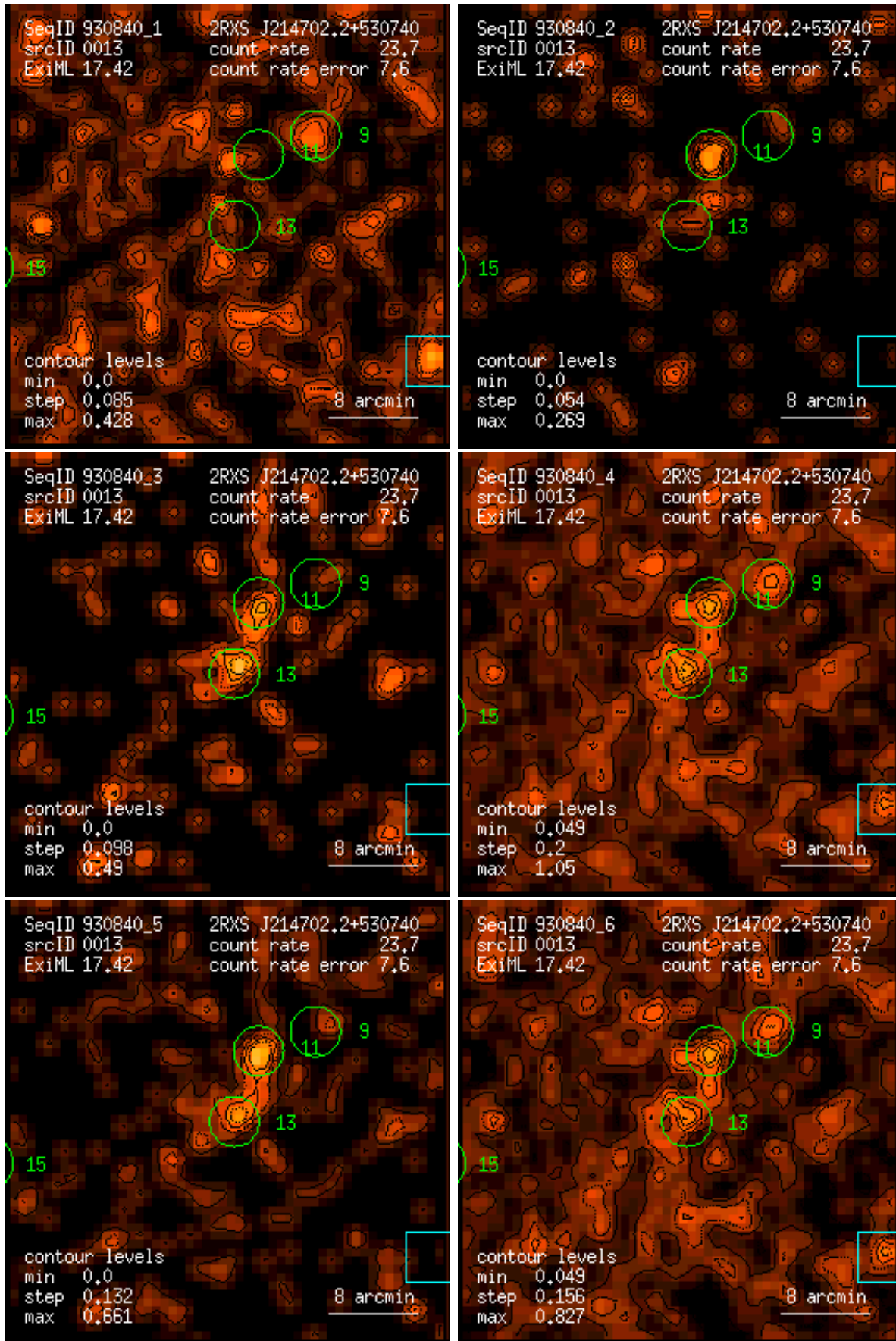
Figure 13: RASS 930840: detection 0013: band rate images, Gaussian filter: (1) PSPC channels 11 – 41, (2) 52 – 90, (3) 91 – 201, (4) 11 – 235, (5) 52 – 201, (6) 11 – 201. Broad band rates in counts/ks. Band rate contour levels in counts/ks/arcmin 2 .
