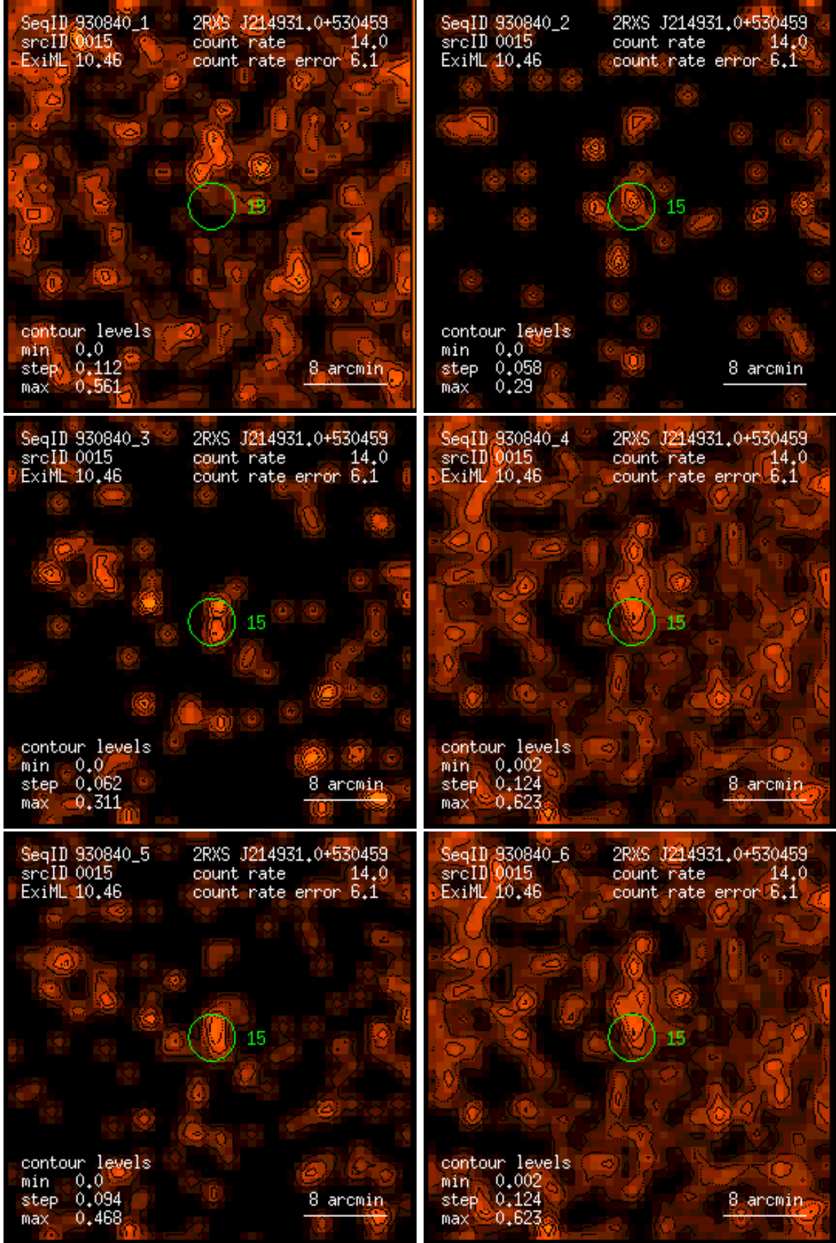
Figure 15: RASS 930840: detection 0015: band rate images, Gaussian filter: (1) PSPC channels 11 – 41, (2) 52 – 90, (3) 91 – 201, (4) 11 – 235, (5) 52 – 201, (6) 11 – 201. Broad band rates in counts/ks. Band rate contour levels in counts/ks/arcmin 2 .
