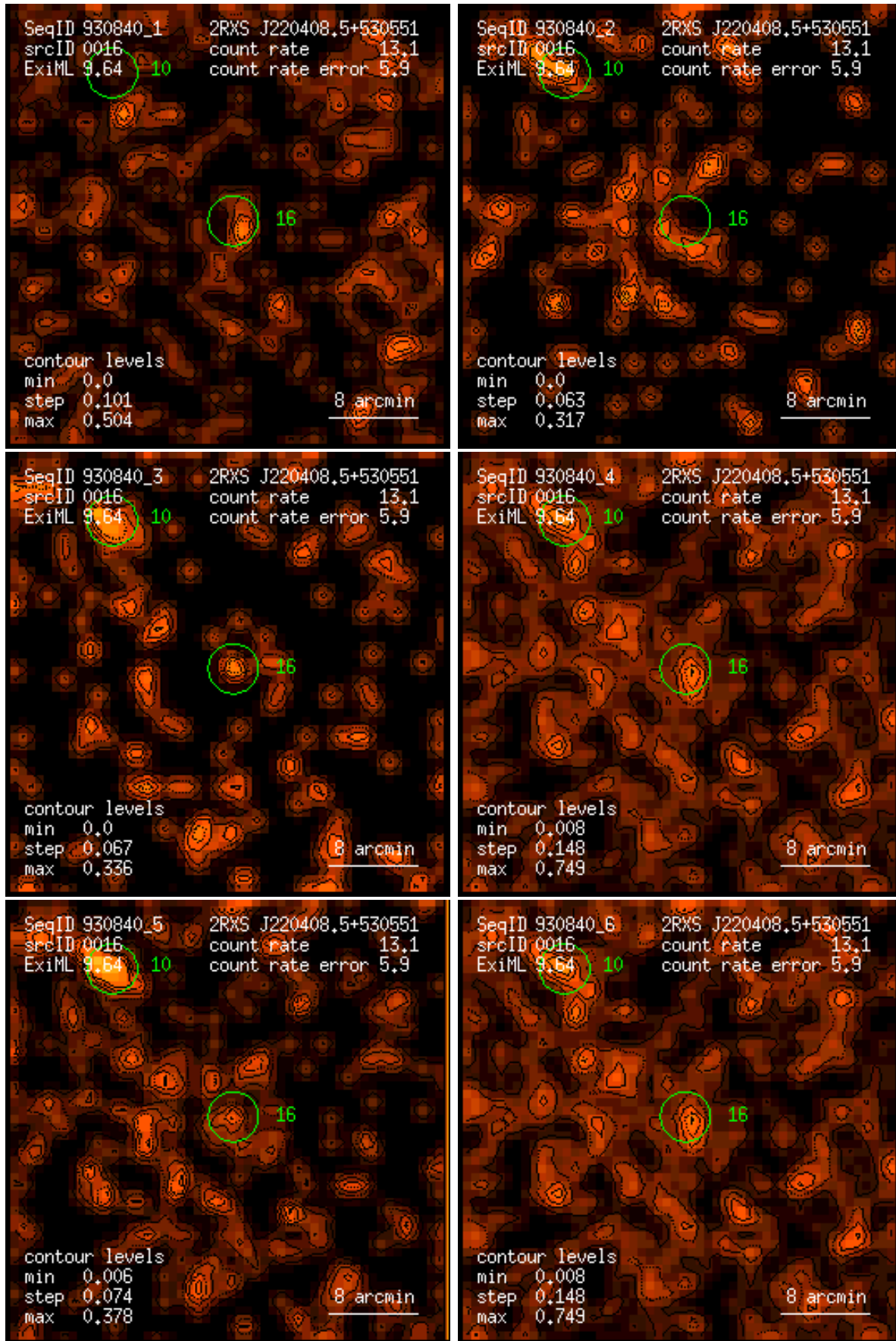
Figure 16: RASS 930840: detection 0016: band rate images, Gaussian filter: (1) PSPC channels 11 – 41, (2) 52 – 90, (3) 91 – 201, (4) 11 – 235, (5) 52 – 201, (6) 11 – 201. Broad band rates in counts/ks. Band rate contour levels in counts/ks/arcmin 2 .
