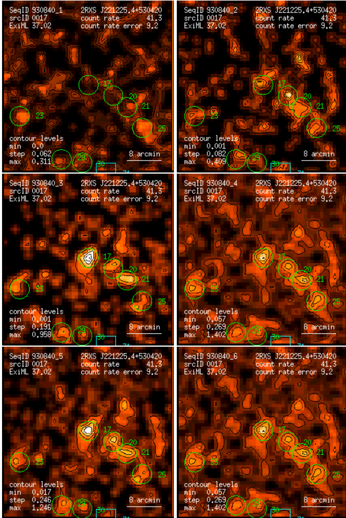
Figure 17: RASS 930840: detection 0017: band rate images, Gaussian filter: (1) PSPC channels 11 – 41, (2) 52 – 90, (3) 91 – 201, (4) 11 – 235, (5) 52 – 201, (6) 11 – 201. Broad band rates in counts/ks. Band rate contour levels in counts/ks/arcmin 2 .
