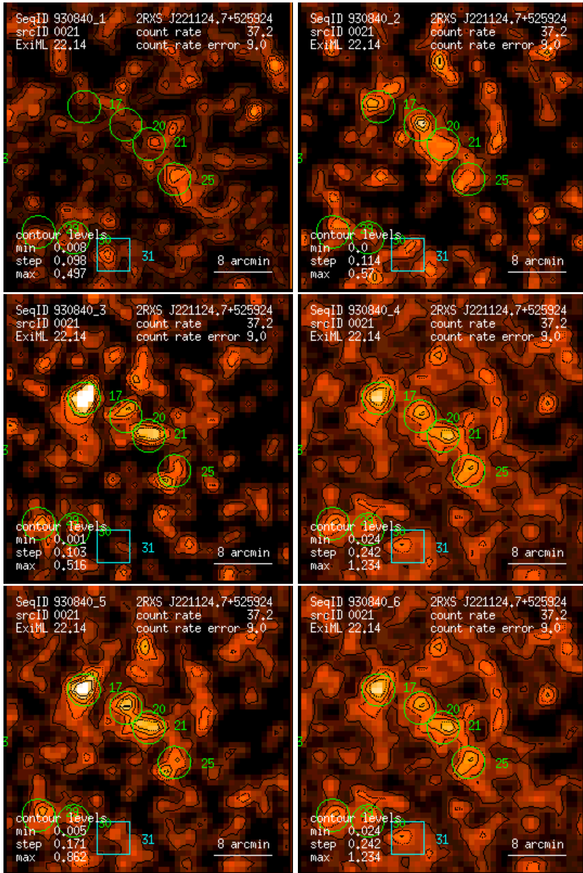
Figure 21: RASS 930840: detection 0021: band rate images, Gaussian filter: (1) PSPC channels 11 – 41, (2) 52 – 90, (3) 91 – 201, (4) 11 – 235, (5) 52 – 201, (6) 11 – 201. Broad band rates in counts/ks. Band rate contour levels in counts/ks/arcmin 2 .
