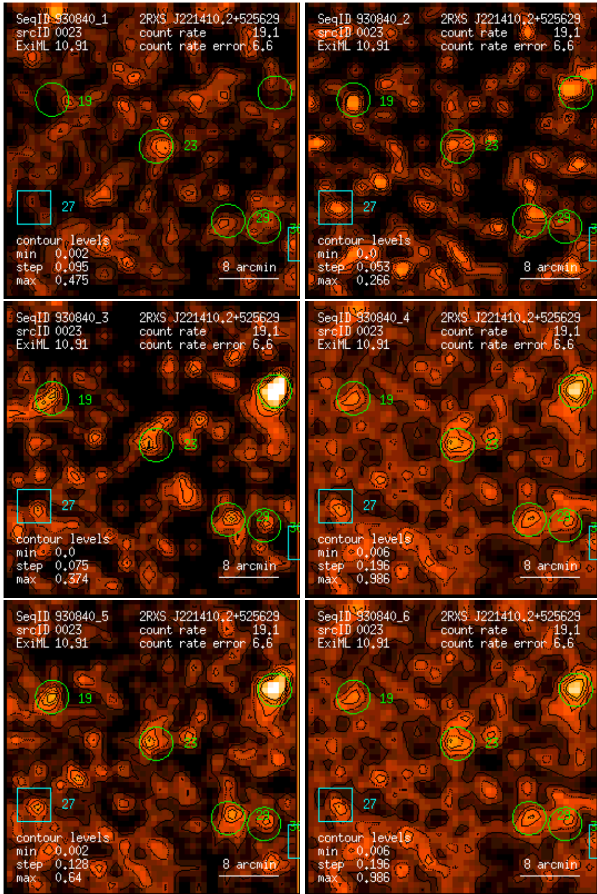
Figure 23: RASS 930840: detection 0023: band rate images, Gaussian filter: (1) PSPC channels 11 – 41, (2) 52 – 90, (3) 91 – 201, (4) 11 – 235, (5) 52 – 201, (6) 11 – 201. Broad band rates in counts/ks. Band rate contour levels in counts/ks/arcmin 2 .
