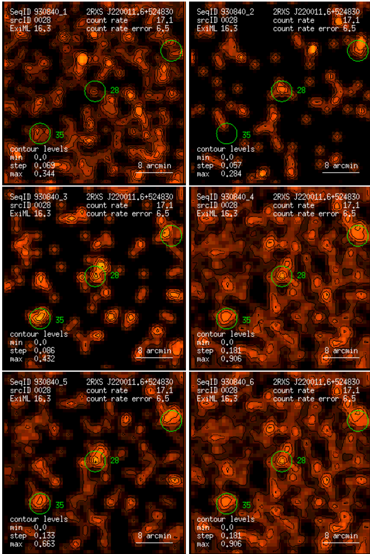
Figure 28: RASS 930840: detection 0028: band rate images, Gaussian filter: (1) PSPC channels 11 – 41, (2) 52 – 90, (3) 91 – 201, (4) 11 – 235, (5) 52 – 201, (6) 11 – 201. Broad band rates in counts/ks. Band rate contour levels in counts/ks/arcmin 2 .
