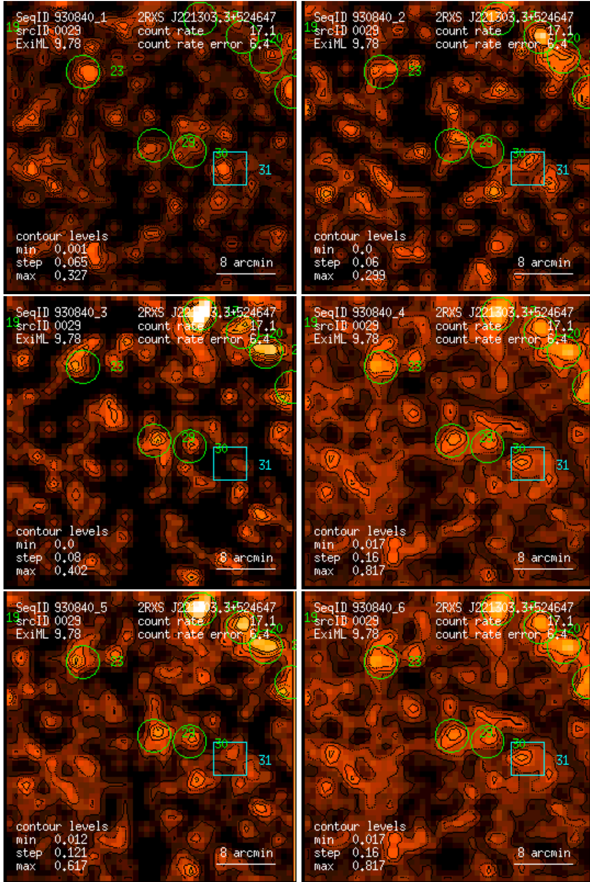
Figure 29: RASS 930840: detection 0029: band rate images, Gaussian filter: (1) PSPC channels 11 – 41, (2) 52 – 90, (3) 91 – 201, (4) 11 – 235, (5) 52 – 201, (6) 11 – 201. Broad band rates in counts/ks. Band rate contour levels in counts/ks/arcmin 2 .
