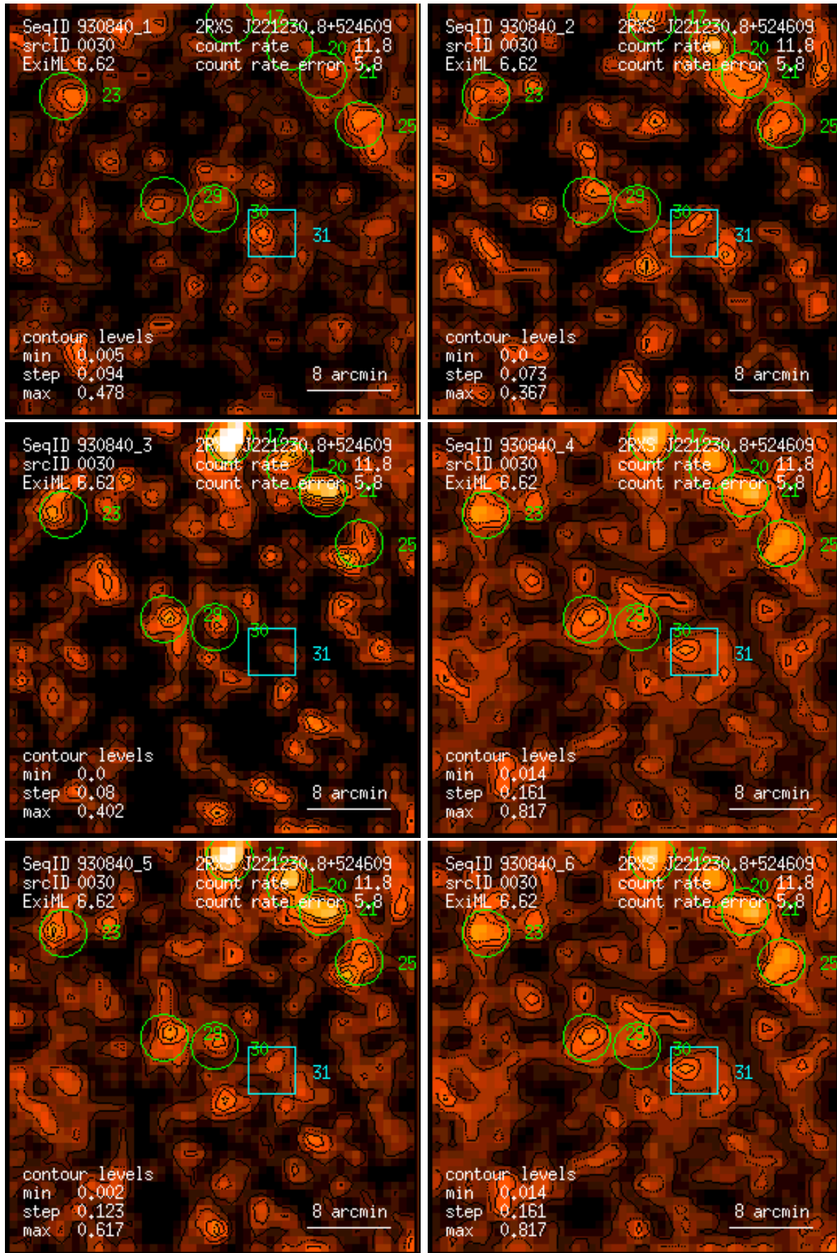
Figure 30: RASS 930840: detection 0030: band rate images, Gaussian filter: (1) PSPC channels 11 – 41, (2) 52 – 90, (3) 91 – 201, (4) 11 – 235, (5) 52 – 201, (6) 11 – 201. Broad band rates in counts/ks. Band rate contour levels in counts/ks/arcmin 2 .
