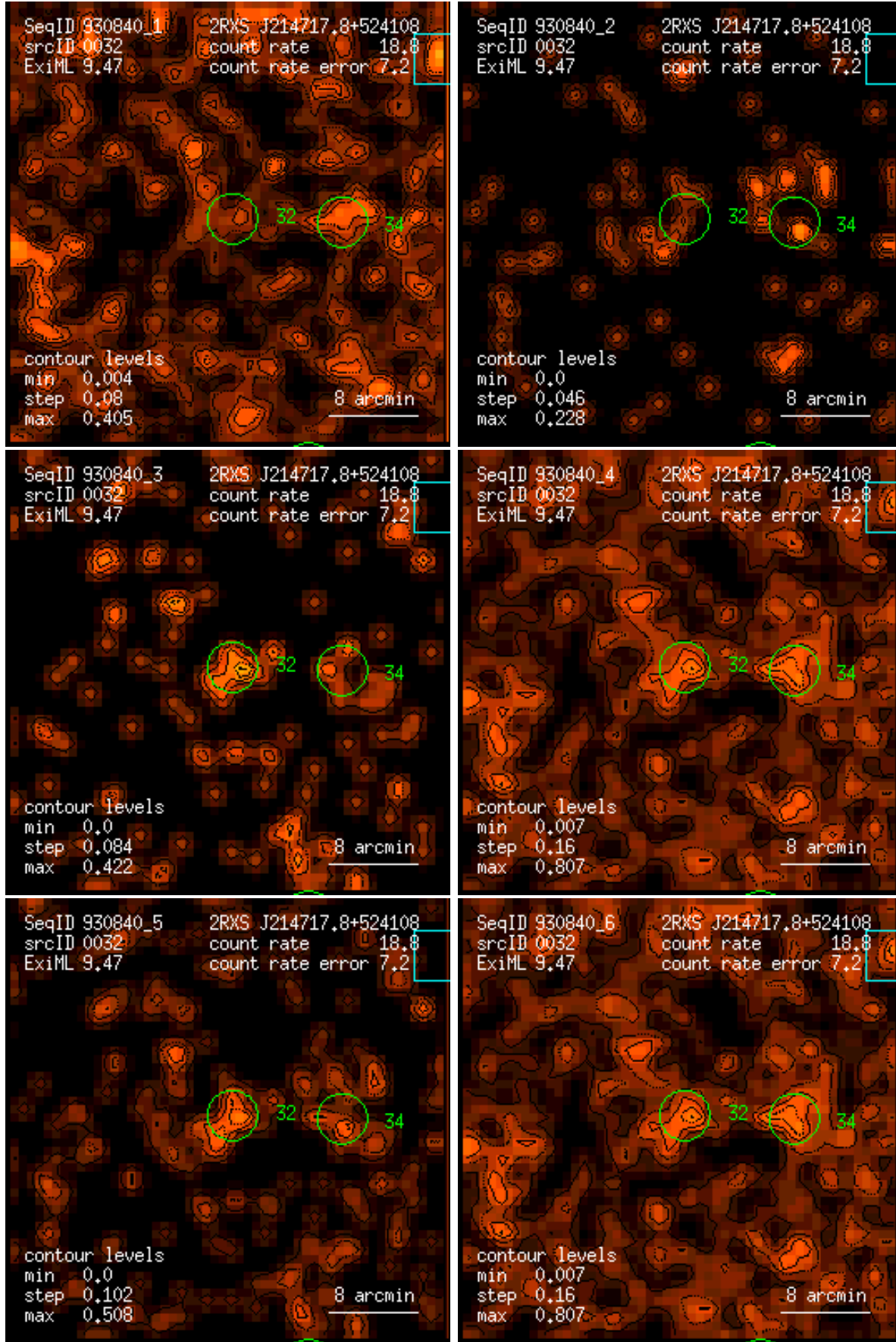
Figure 32: RASS 930840: detection 0032: band rate images, Gaussian filter: (1) PSPC channels 11 – 41, (2) 52 – 90, (3) 91 – 201, (4) 11 – 235, (5) 52 – 201, (6) 11 – 201. Broad band rates in counts/ks. Band rate contour levels in counts/ks/arcmin 2 .
