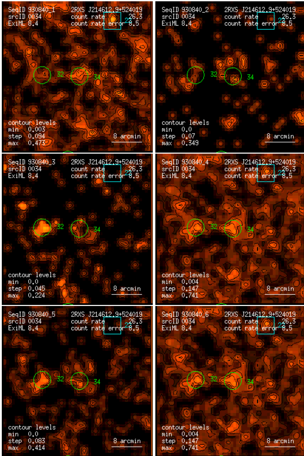
Figure 34: RASS 930840: detection 0034: band rate images, Gaussian filter: (1) PSPC channels 11 – 41, (2) 52 – 90, (3) 91 – 201, (4) 11 – 235, (5) 52 – 201, (6) 11 – 201. Broad band rates in counts/ks. Band rate contour levels in counts/ks/arcmin 2 .
