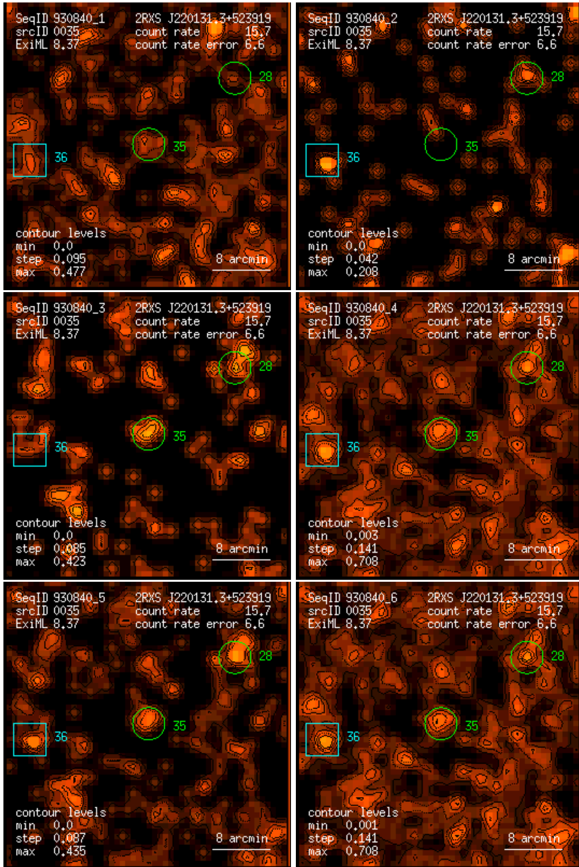
Figure 35: RASS 930840: detection 0035: band rate images, Gaussian filter: (1) PSPC channels 11 – 41, (2) 52 – 90, (3) 91 – 201, (4) 11 – 235, (5) 52 – 201, (6) 11 – 201. Broad band rates in counts/ks. Band rate contour levels in counts/ks/arcmin 2 .
