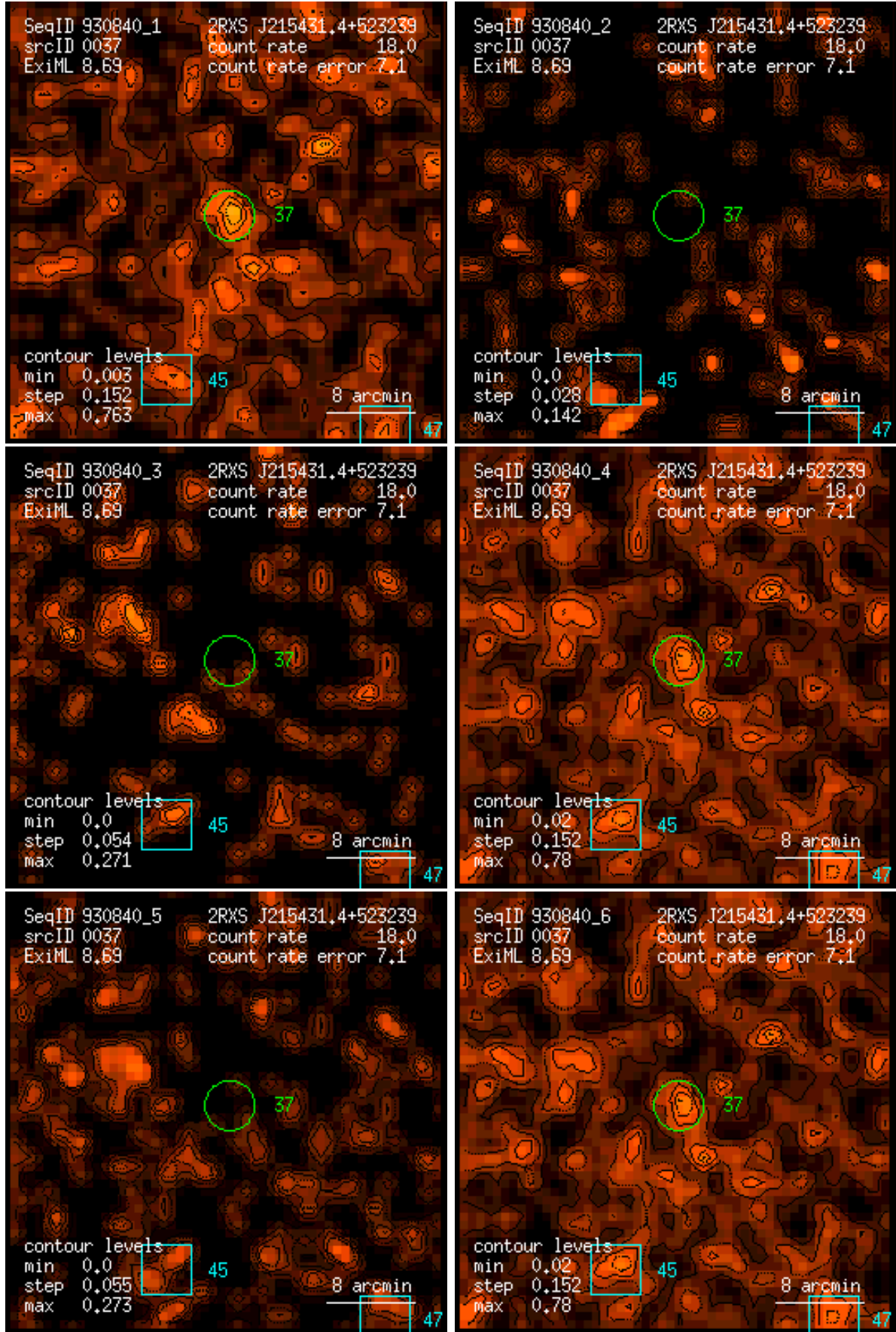
Figure 37: RASS 930840: detection 0037: band rate images, Gaussian filter: (1) PSPC channels 11 – 41, (2) 52 – 90, (3) 91 – 201, (4) 11 – 235, (5) 52 – 201, (6) 11 – 201. Broad band rates in counts/ks. Band rate contour levels in counts/ks/arcmin 2 .
