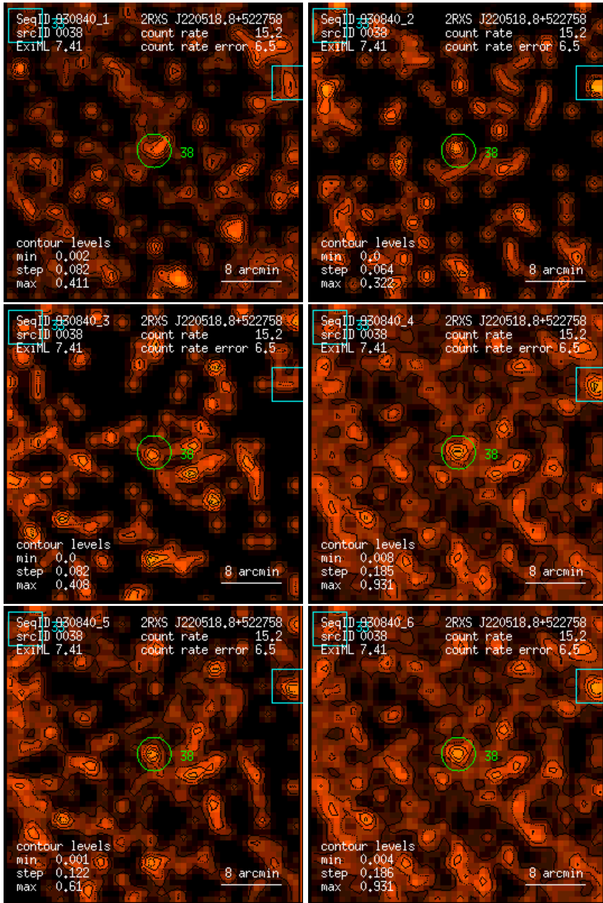
Figure 38: RASS 930840: detection 0038: band rate images, Gaussian filter: (1) PSPC channels 11 – 41, (2) 52 – 90, (3) 91 – 201, (4) 11 – 235, (5) 52 – 201, (6) 11 – 201. Broad band rates in counts/ks. Band rate contour levels in counts/ks/arcmin 2 .
