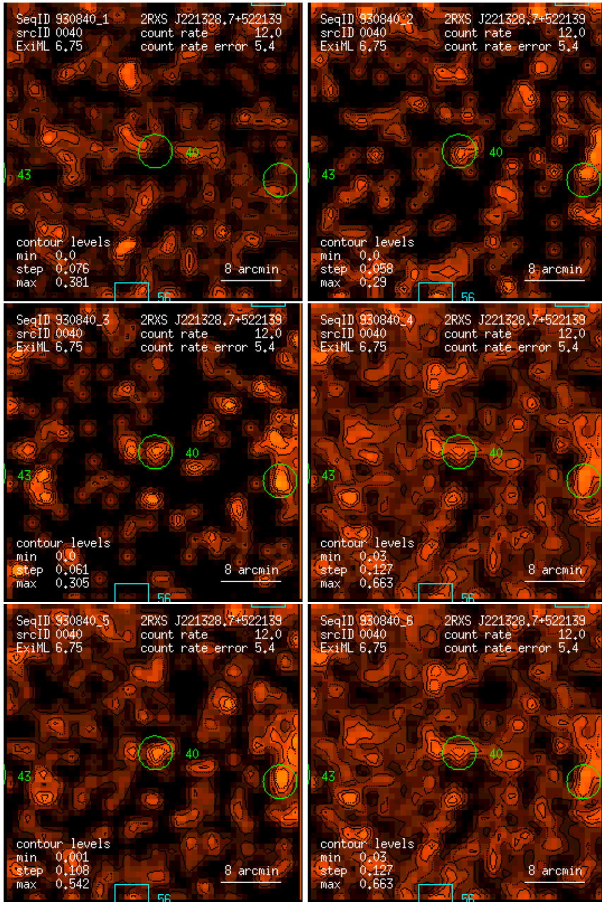
Figure 40: RASS 930840: detection 0040: band rate images, Gaussian filter: (1) PSPC channels 11 – 41, (2) 52 – 90, (3) 91 – 201, (4) 11 – 235, (5) 52 – 201, (6) 11 – 201. Broad band rates in counts/ks. Band rate contour levels in counts/ks/arcmin 2 .
