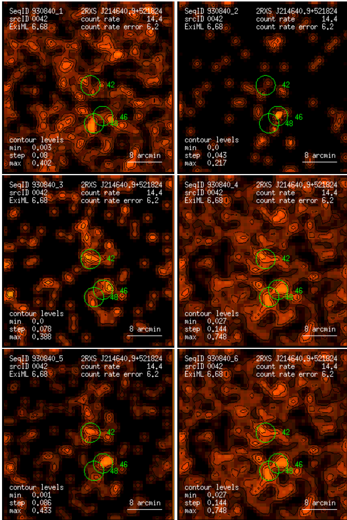
Figure 42: RASS 930840: detection 0042: band rate images, Gaussian filter: (1) PSPC channels 11 – 41, (2) 52 – 90, (3) 91 – 201, (4) 11 – 235, (5) 52 – 201, (6) 11 – 201. Broad band rates in counts/ks. Band rate contour levels in counts/ks/arcmin 2 .
