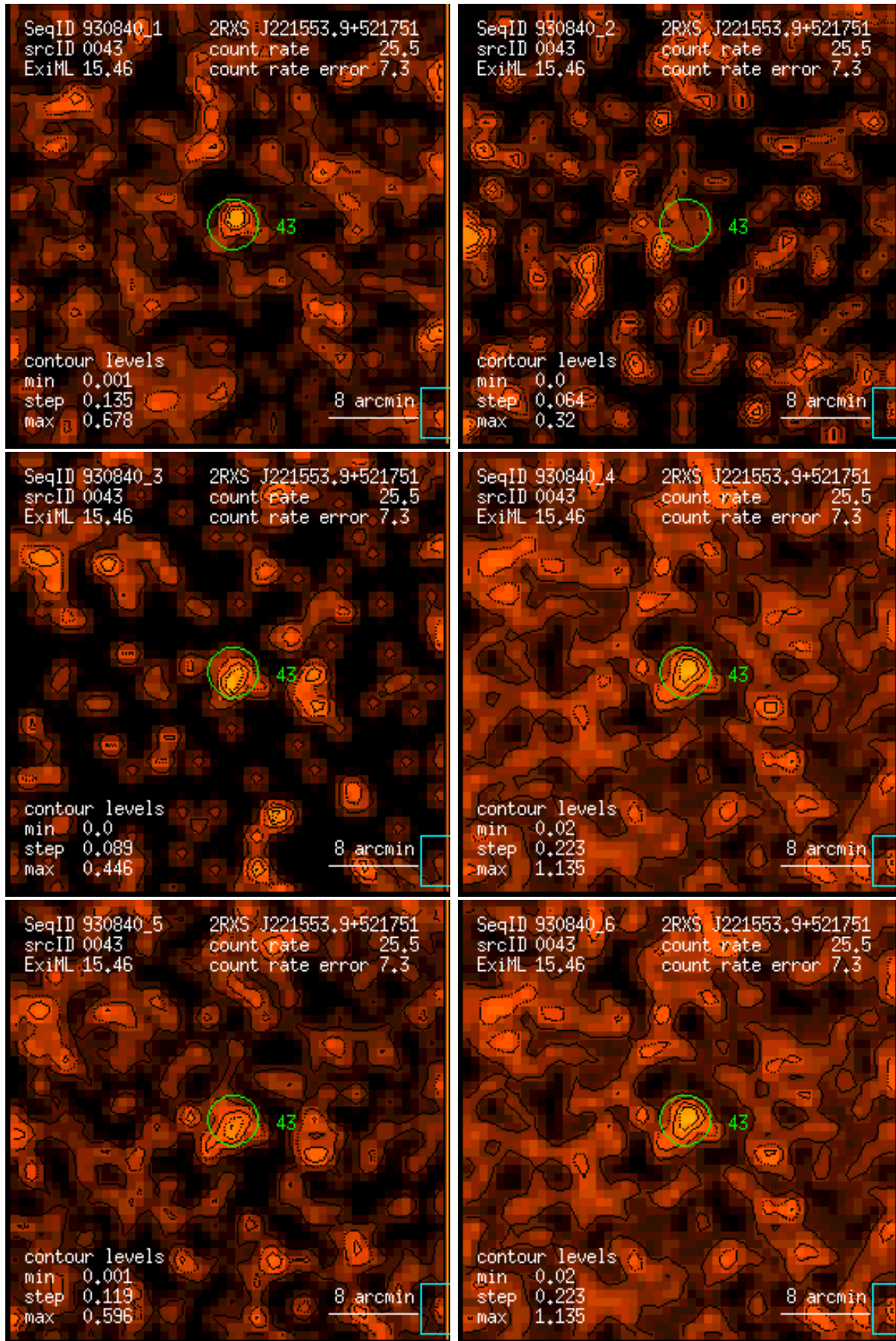
Figure 43: RASS 930840: detection 0043: band rate images, Gaussian filter: (1) PSPC channels 11 – 41, (2) 52 – 90, (3) 91 – 201, (4) 11 – 235, (5) 52 – 201, (6) 11 – 201. Broad band rates in counts/ks. Band rate contour levels in counts/ks/arcmin 2 .
