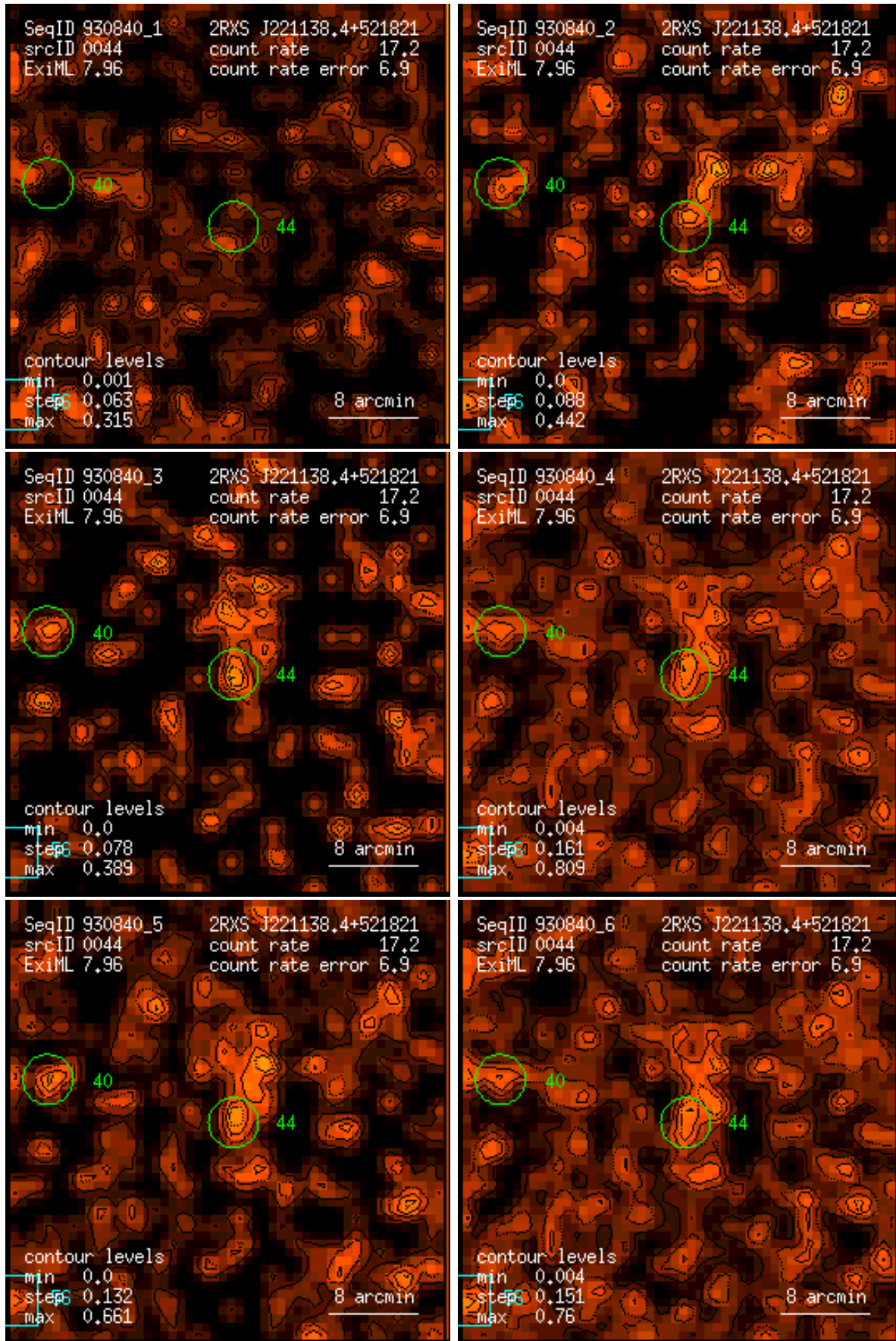
Figure 44: RASS 930840: detection 0044: band rate images, Gaussian filter: (1) PSPC channels 11 – 41, (2) 52 – 90, (3) 91 – 201, (4) 11 – 235, (5) 52 – 201, (6) 11 – 201. Broad band rates in counts/ks. Band rate contour levels in counts/ks/arcmin 2 .
