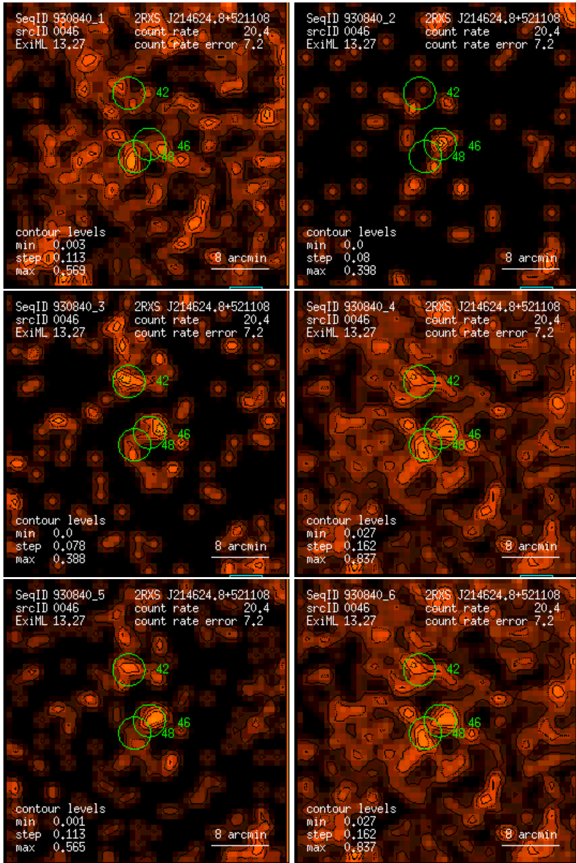
Figure 46: RASS 930840: detection 0046: band rate images, Gaussian filter: (1) PSPC channels 11 – 41, (2) 52 – 90, (3) 91 – 201, (4) 11 – 235, (5) 52 – 201, (6) 11 – 201. Broad band rates in counts/ks. Band rate contour levels in counts/ks/arcmin 2 .
