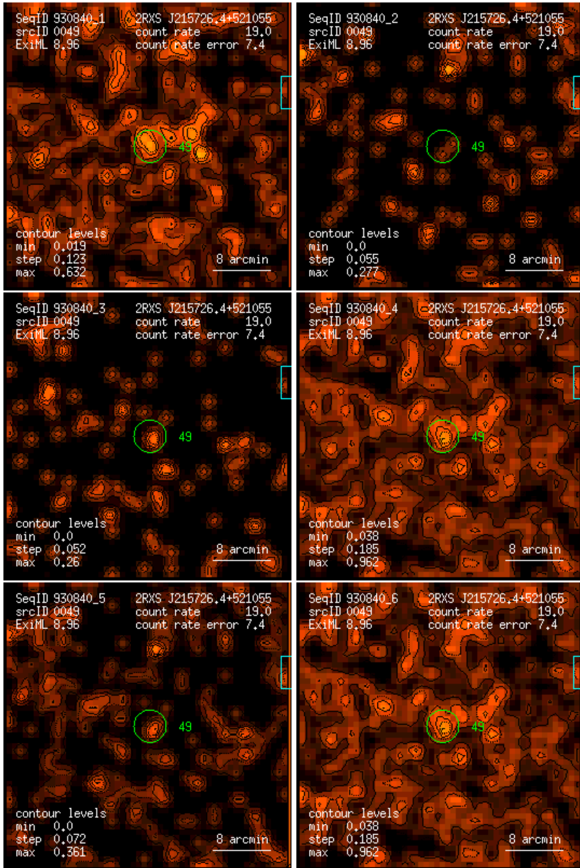
Figure 49: RASS 930840: detection 0049: band rate images, Gaussian filter: (1) PSPC channels 11 – 41, (2) 52 – 90, (3) 91 – 201, (4) 11 – 235, (5) 52 – 201, (6) 11 – 201. Broad band rates in counts/ks. Band rate contour levels in counts/ks/arcmin 2 .
