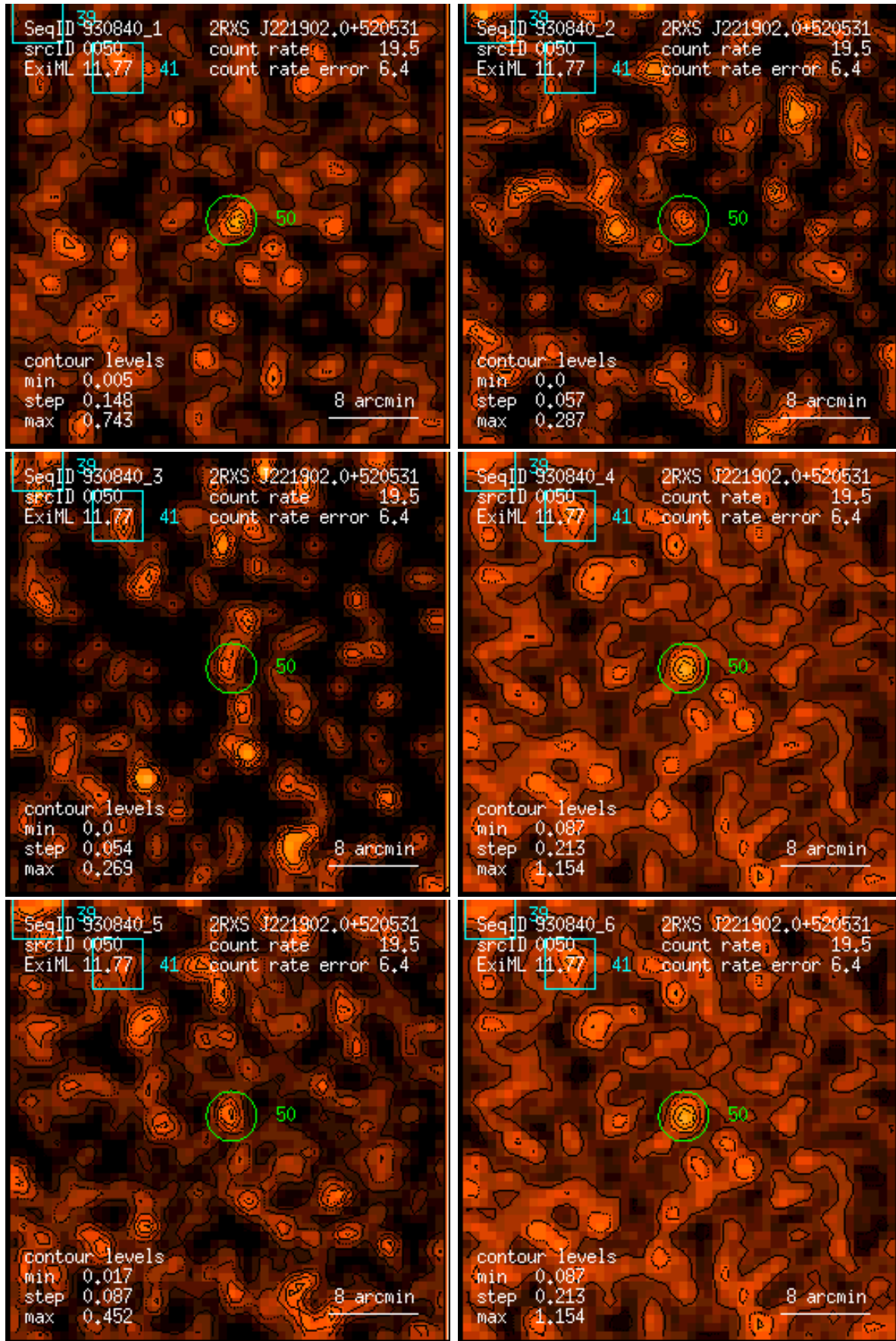
Figure 50: RASS 930840: detection 0050: band rate images, Gaussian filter: (1) PSPC channels 11 – 41, (2) 52 – 90, (3) 91 – 201, (4) 11 – 235, (5) 52 – 201, (6) 11 – 201. Broad band rates in counts/ks. Band rate contour levels in counts/ks/arcmin 2 .
