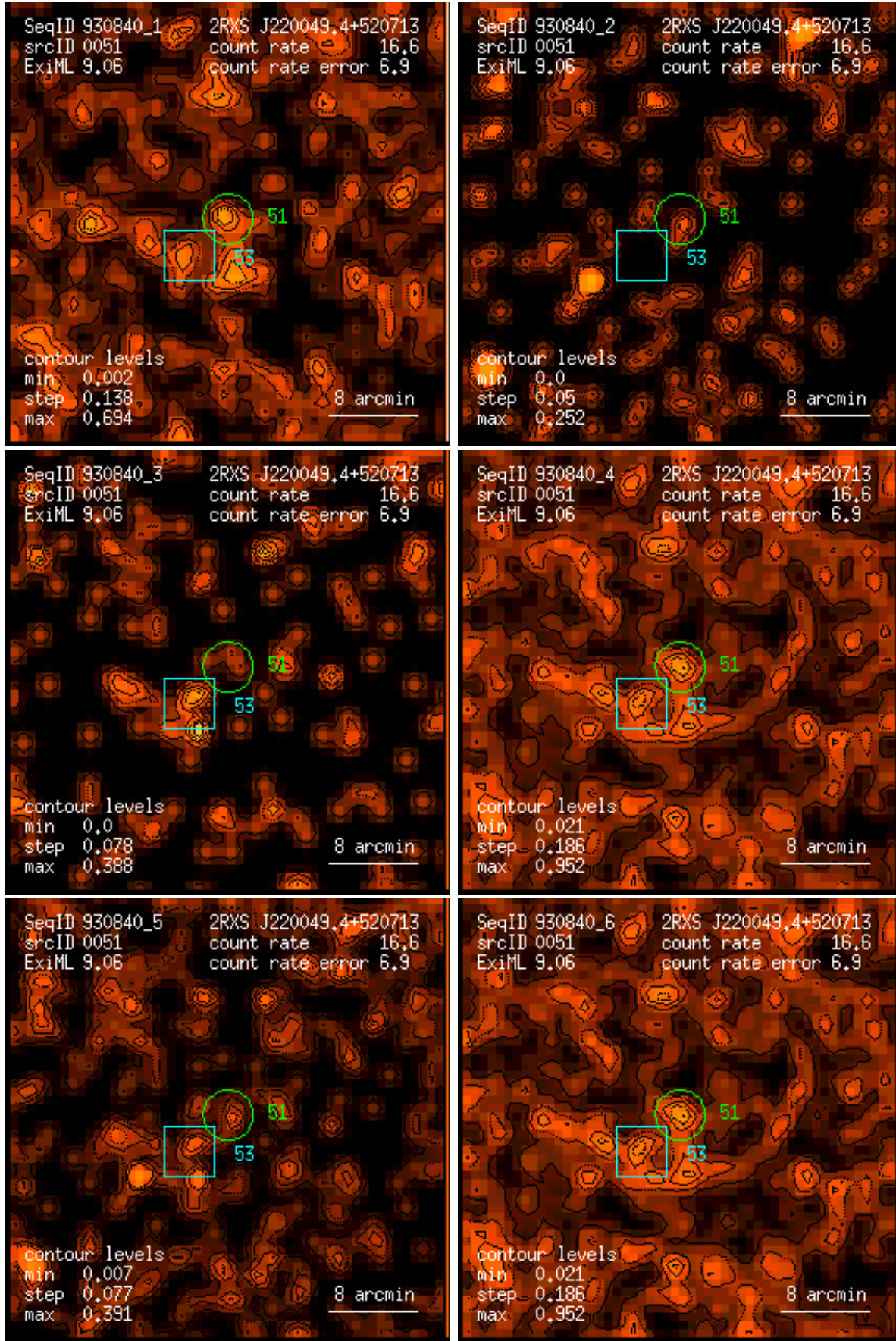
Figure 51: RASS 930840: detection 0051: band rate images, Gaussian filter: (1) PSPC channels 11 – 41, (2) 52 – 90, (3) 91 – 201, (4) 11 – 235, (5) 52 – 201, (6) 11 – 201. Broad band rates in counts/ks. Band rate contour levels in counts/ks/arcmin 2 .
